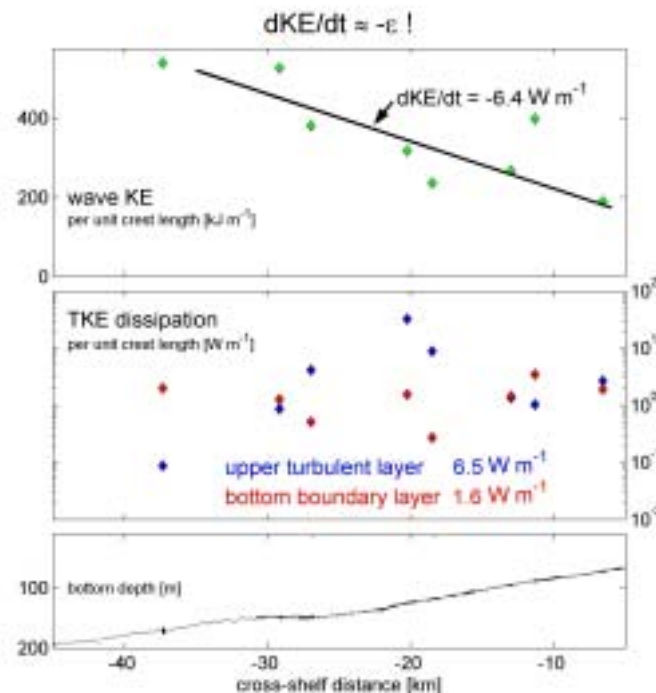
Figure 2 – Evolution of the observed wave as it propagated 30 km onshore during a 12 h period (mean phase speed, 0.7 m/s). The wave kinetic energy (top panel) decreased by a factor of 5, or at the rate -6.4 \text{ W} per unit crest length. This is nearly equal to the mean value of the turbulent dissipation rate measured in the wave during the 8 profiling transects (2 nd panel, blue).
