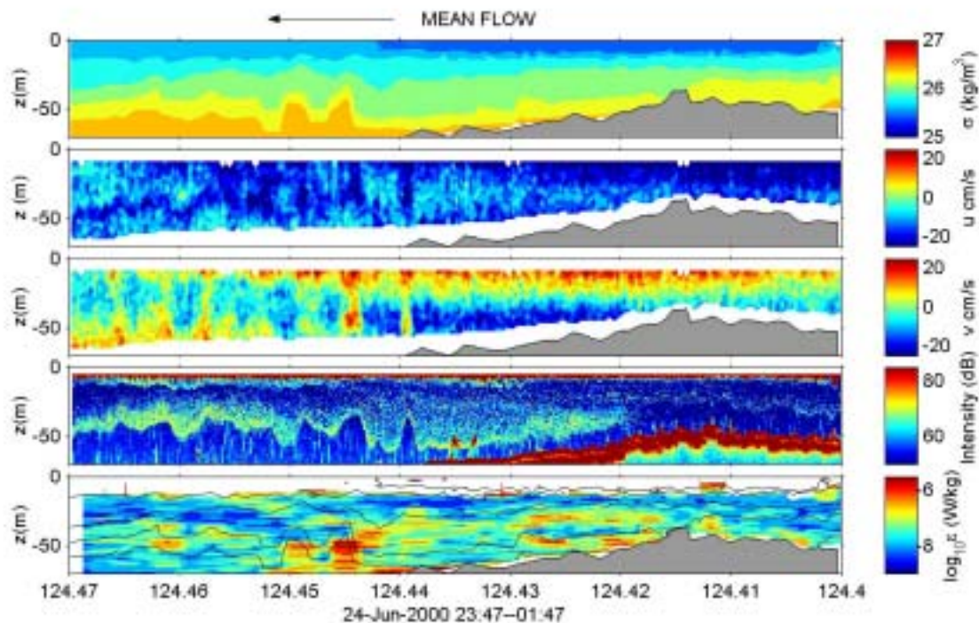
Figure 3 – One of 28 transects across Stonewall Bank in June 2000. The top panel shows density as determined from CHAMELEON, the 2nd panel is the cross-bank current and the 3 rd panel is the along-bank current. The 4 th panel is the acoustic backscatter from a high frequency echosounder mounted in the hull of the ship (Farmer) and the bottom panel is the turbulent dissipation rate with density contours. The total length of this transect is 8 km. Bottom is shaded gray in all panels except the echosounder intensity in which the bottom is indicated by the high backscattering strength (red). The downstream wake includes large amplitude waves west (to the left of) 124.44 W.
