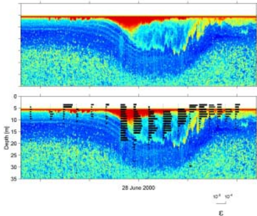
Figure 1 – CHAMELEON profiles indicate strong turbulence within the wave structure, which is clearly outlined by acoustic backscatter. These were made with the ship drifting and the wave propagating shoreward (right to left) past the ship. Profiles do not line up exactly with the acoustic image due to relative motion of ship and CHAMELEON during the profile.
