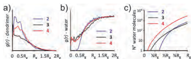
Fig. 2 Radial distribution functions, g(r) , obtained from the equilibrated phase MD simulations. The g(r) curves are indicative of the probability to find atoms of the dendrimers (a) and water molecules (b) at given distance from the dendrimer's center of mass (CM). (c) Number of water molecules.
