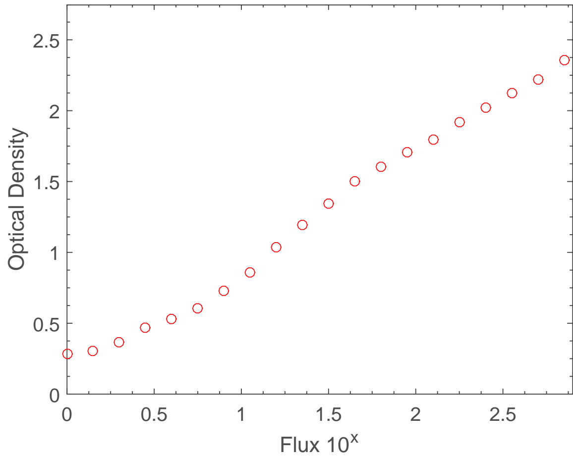
Figure 6. Example of an MF HD curve derived from a step wedge.
