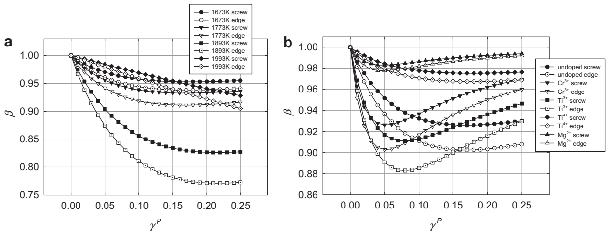
Fig. 9. Predicted cumulative heat dissipation fraction from slip on the basal plane: (a) pure alumina over range of temperatures and (b) pure and doped alumina at \theta \approx 1800 \text{ K} .
