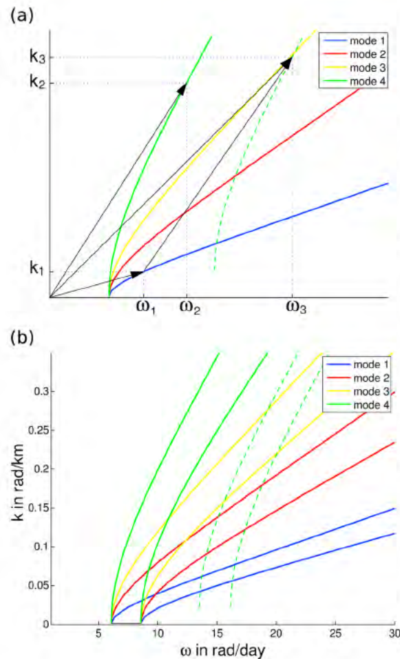
Figure 4. Sketch of internal wave wave triad interactions in K\omega space. (a) The dispersion relations of four internal wave vertical modes. The cross section of the green dashed and yellow lines illustrates the triad interaction, where mode 1 and mode 4 internal waves form a mode 3 internal wave with the frequency \omega_3 and wave number k_3 . (b) Equivalent approach as in Figure 4a but applied to a band of internal wave dispersion relations given by a range of geographical latitudes and vertical stratification profiles.
