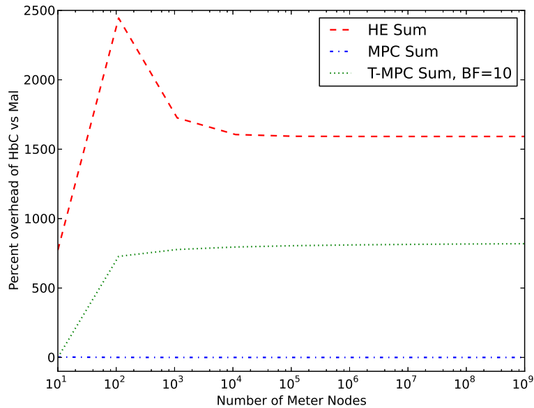
Figure 5.5: Percent overhead for HbC vs Malicious when computing summation.
