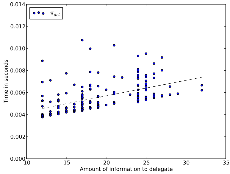
Figure 4.15: Timing as amount of information increases for \pi_{del} .
