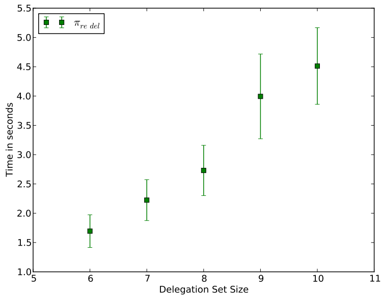
Figure 4.14: Average time to execute \pi_{re del} with varying delegation set size and 95% confidence interval.
