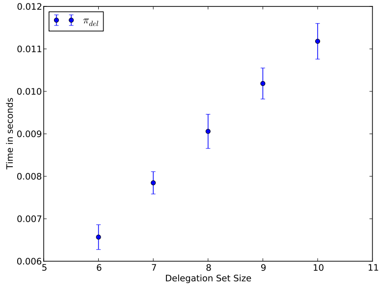
Figure 4.13: Average time to execute \pi_{del} with varying delegation set size and 95% confidence interval.
