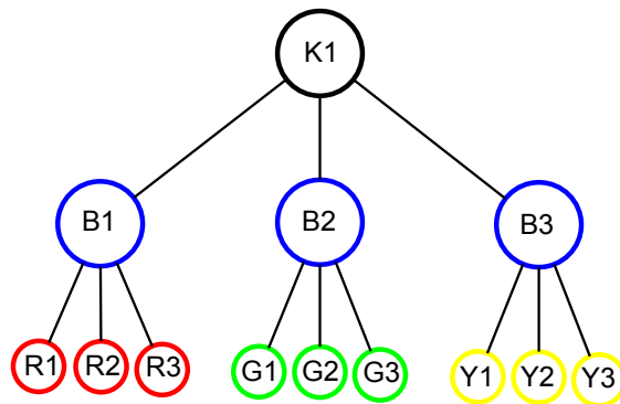
Figure 4.1: Applying transferable multiparty computation to a tree structured network.
