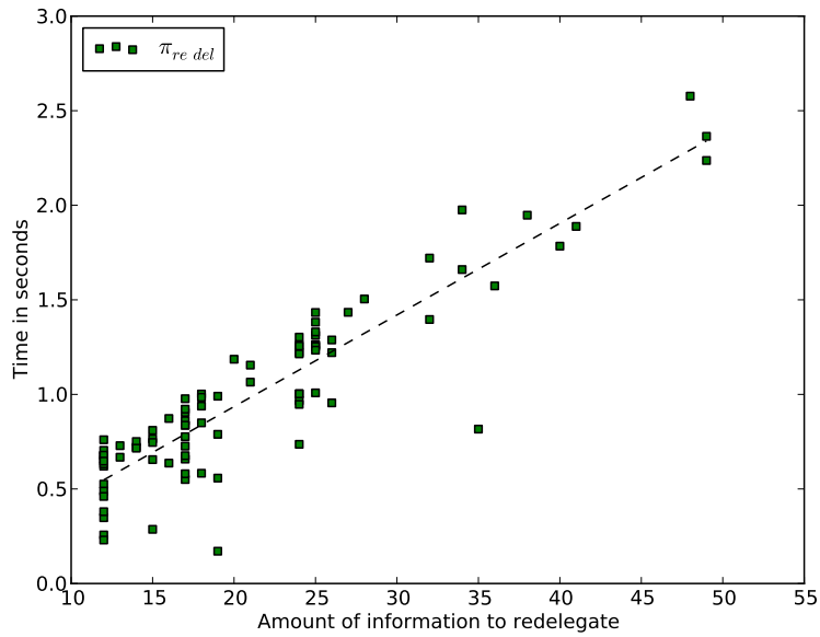
Figure 4.16: Timing as amount of information increases for \pi_{re del} .
