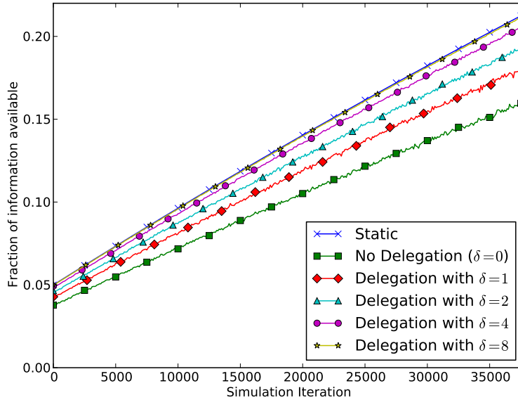
Figure 4.7: Information availability for various delegation depths ( a = 0.75 ).
