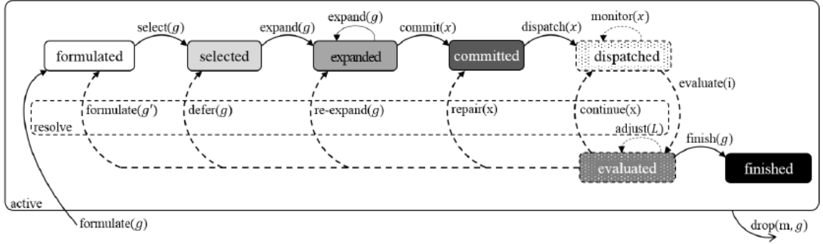
Figure 1: The goal lifecycle [12]
