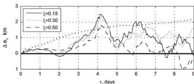
Fig. 5. Difference \Delta e_\tau between the forecast errors of the 2dVar interpolated HFR fields obtained with W_d = 0 and W_d \neq 0 with various values of the gap concentration parameter \xi . 70% confidence limit for the difference is shown by the thick dotted line. Positive values correspond to smaller forecast error of the divergence-penalizing interpolation ( W_d \neq 0 ).
