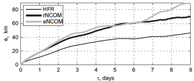
Fig. 7. Drifter forecast error e_r for the results of 2dVar interpolation of HFR data with enforced smoothness in the divergence field (black curve) and for the NCOM model solutions shown by thick lines.
