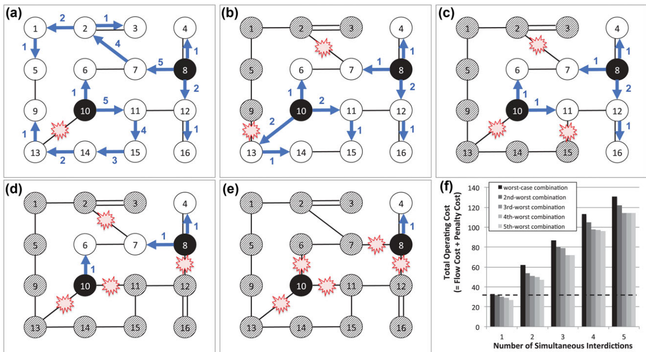
Fig. 3. Worst-case simultaneous interdictions. (a) The worst-case single interdicted link is of link [10, 13], resulting in a total cost of 33. In this case, the flow cost increases but all nodes are still served. (b) The worst-case simultaneous two-link interdicted link is of links [2, 7] and [9, 13], which denies nodes 1, 2, 3, 5, and 9 (now shaded) any flow. The total cost is 62 ( =12 + 50 ), most of which is unmet demand penalty cost. (c) The worst-case simultaneous three-link interdicted link is of links [2, 7], [10, 13], and [11, 15], resulting in a total cost of 87 ( =7 + 80 ). (d) The worst-case simultaneous four-link interdicted link is of links [2, 7], [8, 12], [10, 11], and [10, 13], resulting in a total cost of 113 ( =3 + 110 ). (e) The worst-case simultaneous five-link interdicted link is of links [6, 10], [7, 8], [8, 12], [10, 11], and [10, 13], resulting in a total cost of 131 ( =1 + 130 ). (f) The worst-case (rank 1) attack for 1–5 simultaneous interdictions increases approximately linearly. The second-worst (rank 2) through fifth-worst (rank 5) attacks do less damage, but all are significantly worse than the baseline (no interdicted) case that has operating cost 25.
