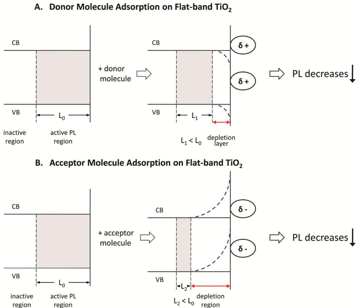
Figure 11. Schematic effect of donor and acceptor molecules on the thickness of the active PL region. A. \text{TiO}_2 with flat-band condition achieved by maximum UV exposure in vacuum. The active PL region length = L_0 . Upon adsorption of an electron donor molecule the active PL region decreases to L_1 where L_1 < L_0 resulting in the PL intensity decrease; B. After adsorption of an electron acceptor molecule the length of the active PL region narrows ( L_2 < L_0 ) leading to PL intensity decrease.
