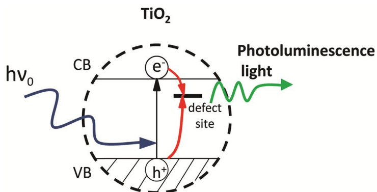
Figure 15. Schematic of photoluminescence process. Recombination of photo-excited charge carriers at a defect site result in emission of photoluminescence light.
