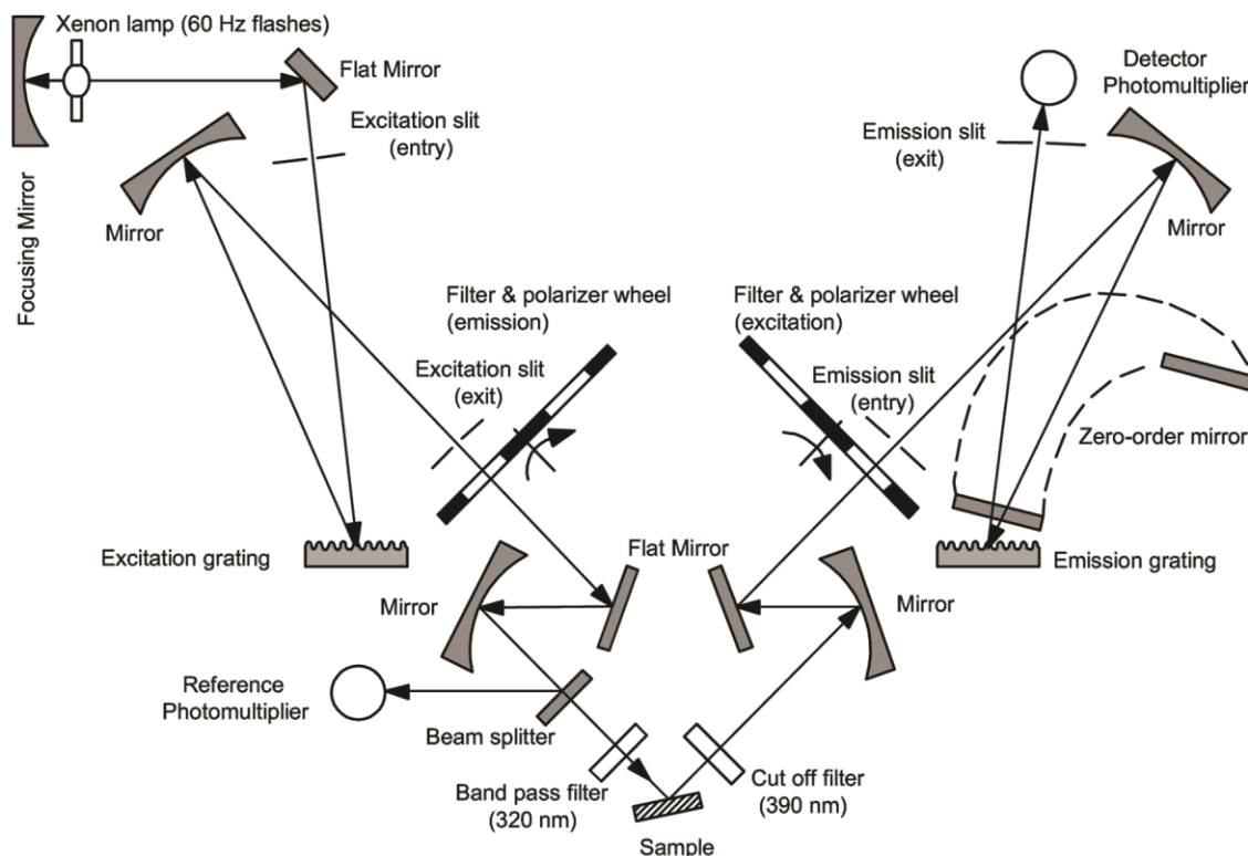
Figure 16. Schematic representation of a standard photoluminescence instrument that employs right-angle detection geometry. The standard instrument is modified by a 320 nm band pass filter and a 390 nm cut off filter.
