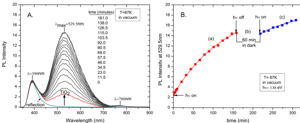
Figure 2. A. Photoluminescence development of TiO 2 during irradiation in vacuum. Reference spectrum, a clean W-grid at the sample position, is shown by the blue line. B. The photoluminescence intensity of TiO 2 increases as a function of UV exposure at 87 K in vacuum: (a) The sample was irradiated by \lambda=3.88 eV for 160 min (red curve). The photoluminescence intensity increases with irradiation as the number of photon-accessible defects increases; (b) The sample was stored in the dark in vacuum for 60 min; (c) The sample was irradiated again by \lambda=3.88 eV for 90 min. (blue curve). Photoluminescence remains constant when the UV light is off (~60 min) and continues to increase when the UV light is on.
