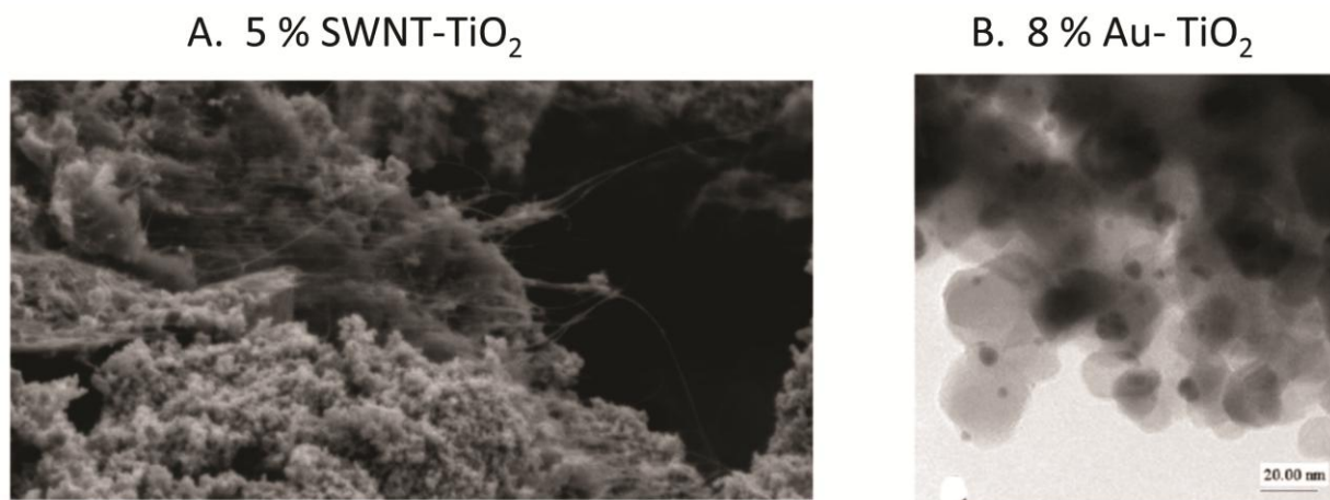
Figure 2. TEM Micrograph of A. 5 % SWNT-TiO 2 composite; B. 8 % Au- TiO 2 composite.
