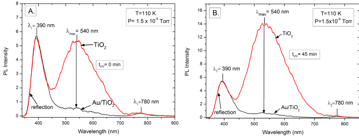
Figure 5. Photoluminescence spectra of pure \text{TiO}_2 (red spectra) and \text{Au/TiO}_2 (gray spectra) in vacuum at 110 K. The PL emission shows maximum at \sim 540 nm when excited by 320 nm (3.88 eV) light. A. PL spectra before UV irradiation; B. PL spectra after 45 min of continuous UV irradiation. The PL intensity of \text{TiO}_2 is significantly suppressed in the \text{Au/TiO}_2 sample. The peak at 390 nm and a second-order feature at 780 nm is due to reflection of the incident light from both \text{CaF}_2 window and the tungsten grid.
