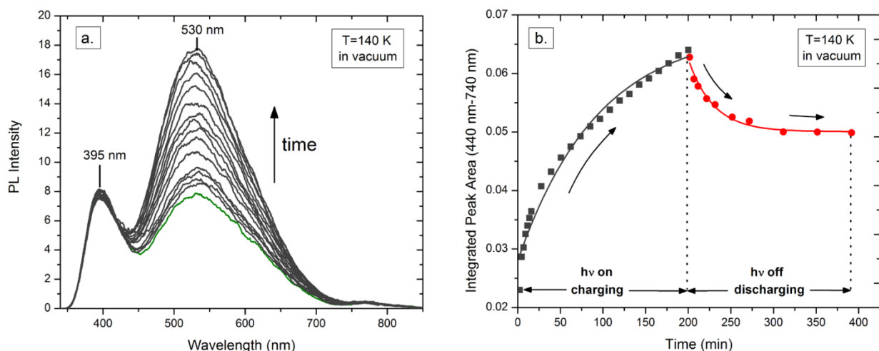
Figure 2. a. Development of a 530 nm \text{TiO}_2 photoluminescence feature during continuous UV irradiation in vacuum at 140 K. b. Change in PL intensity during and upon discontinuation of UV irradiation in vacuum at 140 K: Gray curve shows an exponential increase in PL intensity upon irradiation of \text{TiO}_2 particles indicating a decrease in the surface negative charge due to electron hopping from particle to particle, charging the interior of the \text{TiO}_2 network. The red curve shows a decrease in the PL intensity of the \text{TiO}_2 particles as negative charge transports from the interior of the \text{TiO}_2 powder back to the surface, partially restoring upward band bending.
