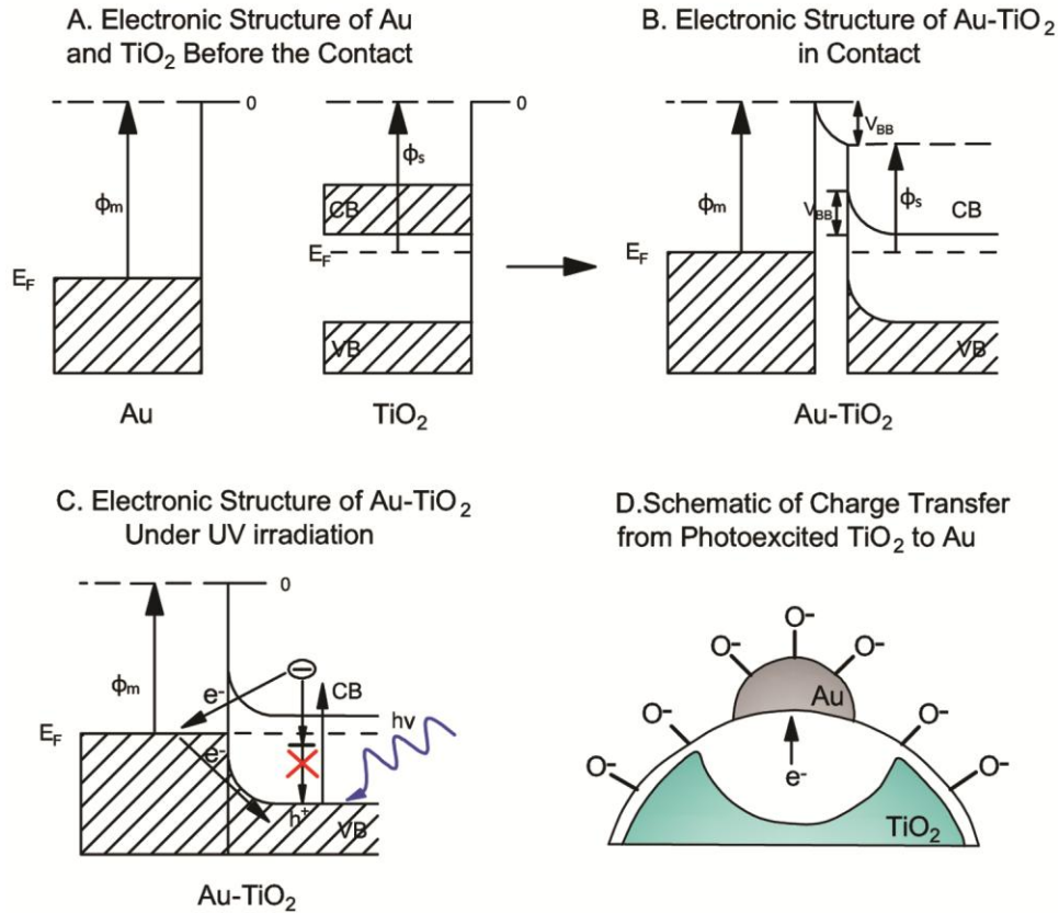
Figure 7. A. Electronic structure of Au and \text{TiO}_2 before the contact; B. Electronic structure of Au and \text{TiO}_2 after the contact; C. Electronic structure of Au - \text{TiO}_2 upon photoexcitation of \text{TiO}_2 . Gold nanoparticles are capable of accepting negative surface charge and also electrons from the conduction band resulting in suppressed PL signal. Possible channel for the Au nanoparticles to discharge is through recombination of trapped electrons in the Au particles with holes in \text{TiO}_2 . This recombination process results in heat emission; D. Schematic of photoexcited charge withdrawal from \text{TiO}_2 to Au nanoparticles.
