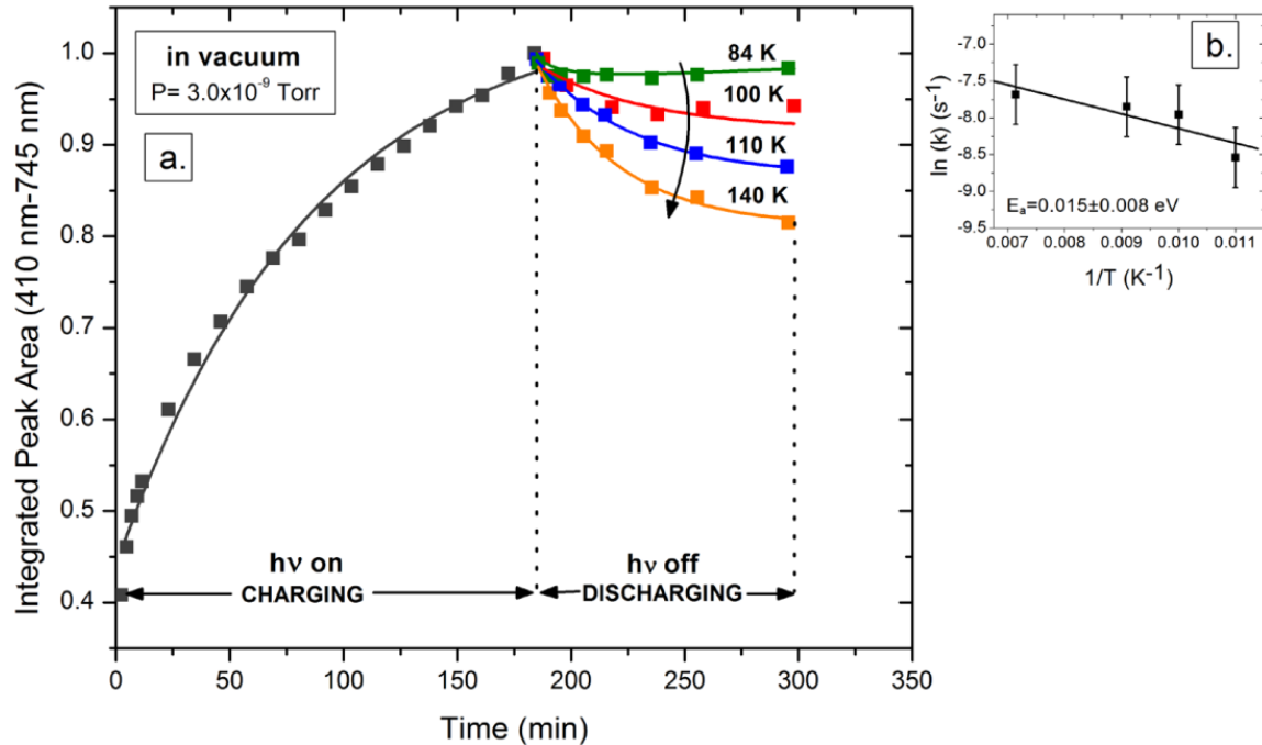
Figure 5. Photoluminescence decay in the dark in vacuum at different temperatures. Gray points represent the PL development upon UV irradiation. The \text{TiO}_2 surface is prepared to a near-flat band condition as a saturation PL intensity plateau is almost achieved. Upon interruption of UV light, the PL decrease is observed at different temperatures: 84 K (green); 100 K (red); 110 K (blue) and 140 K (orange). Inset b. shows the natural logarithm of the rate of charge migration in the dark as a function of temperature where the extracted activation energy is 0.015 \pm 0.008 \text{ eV} . The data are normalized at the maximum PL intensity.
