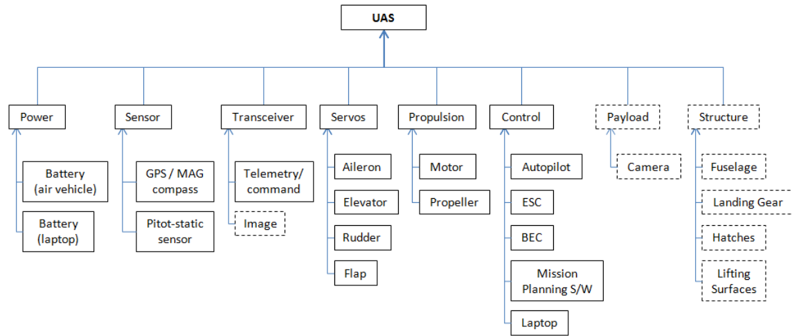
Figure 24: Functional Grouping of Components in FMECA
