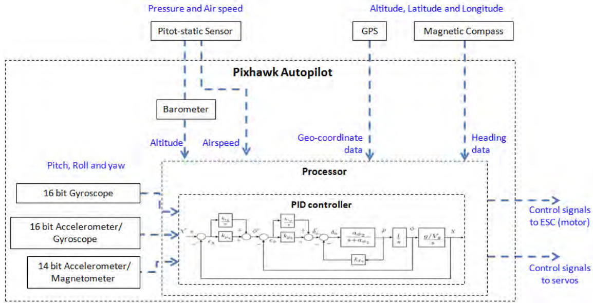
Figure 10: Schematic of “ Pixhawk Autopilot ” for State Variable of Motion
