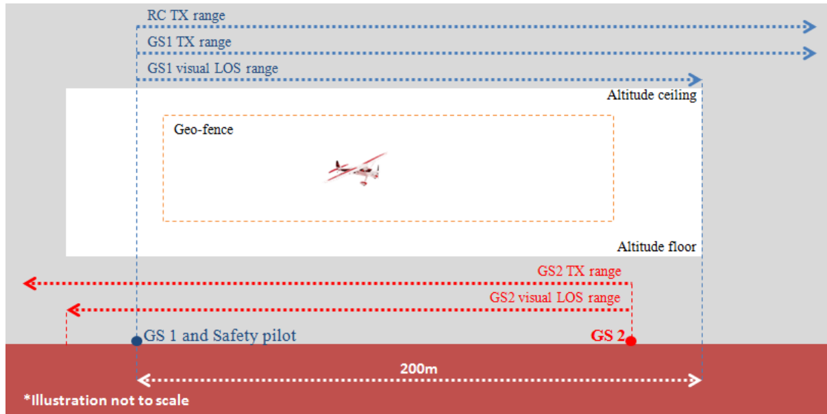
Figure 30: Airspace Envelope for Flight Test
