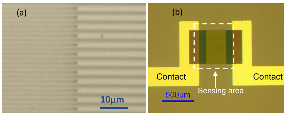
Figure 10: Optical images of (a) electrode features after e-beam lithography with PMMA e-beam resist and (b) the impedance sensor after fabrication
