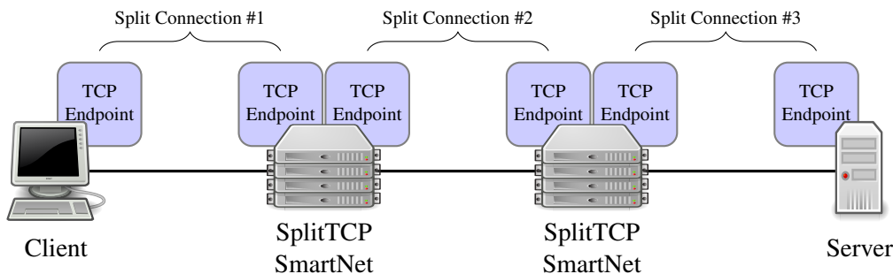
Figure 4.5: End-to-end connection using SplitTCP plugin. The SplitTCP plugin divides the end-to-end TCP connection in to several hop-by-hop TCP connections.
