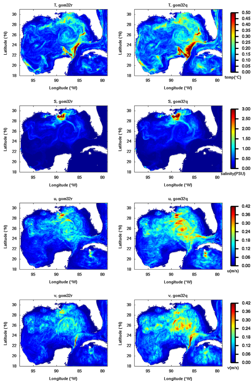
Fig. 3. Initial ensemble spread for r (left panel) and q (right panel) at 00UTC July 17, 2012 at the surface for temperature, salinity, u , and v (from top to bottom).
