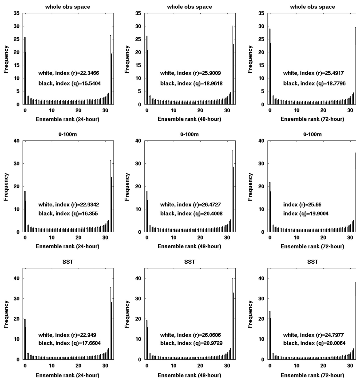
Fig. 9. Talagrand rank histograms for temperature ( r : white, q : black) using observation as truth for lead times of 24, 48, and 72 h (from left to right). All the values are averaged over the 109 days period from June 1 to September 17, 2012, and over the full observation space (top panel), the layer between 0 and 100 m (middle panel), and the surface (bottom panel). Consistency index is also indicated in each case for both ensembles.
