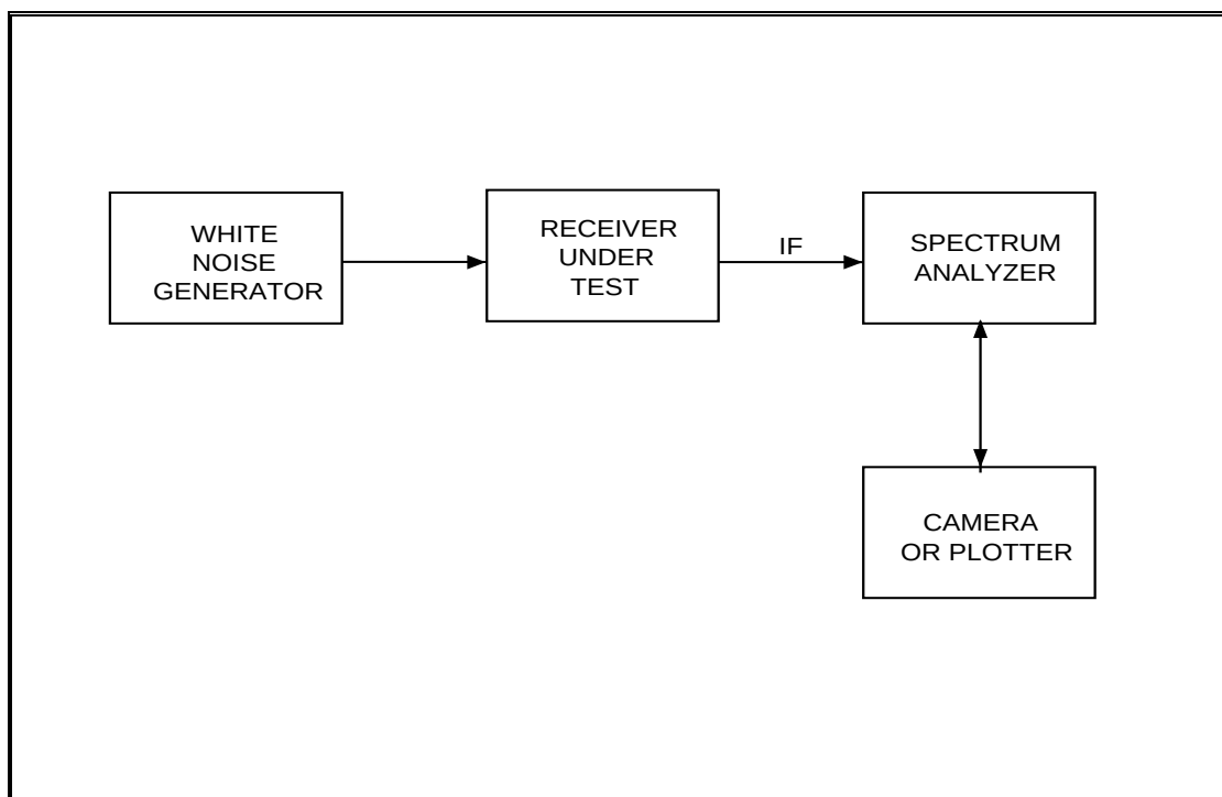
Figure 4-17. Receiver band pass response using white noise (see test 4.15).
