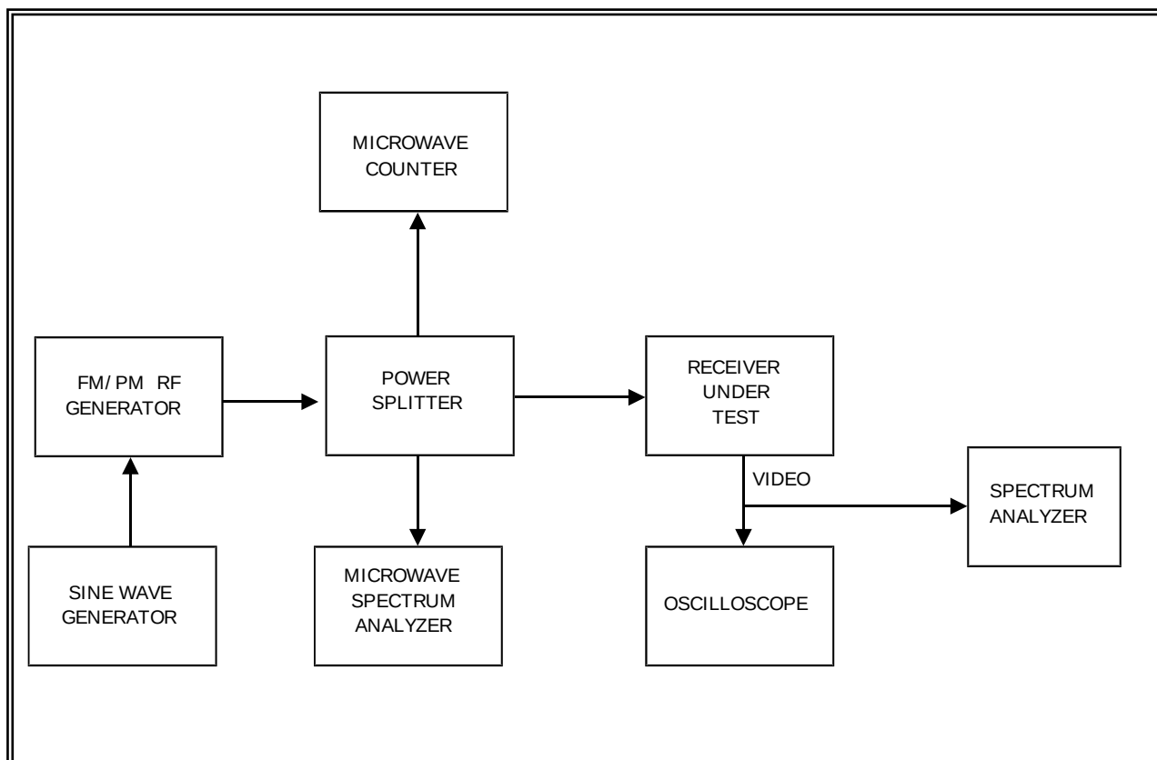
Figure 4-20. Receiver video spurious outputs (see test 4.18)
