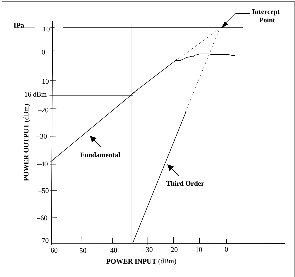
Figure 2-7. Graphical illustration of intercept point (see test 2.3).
