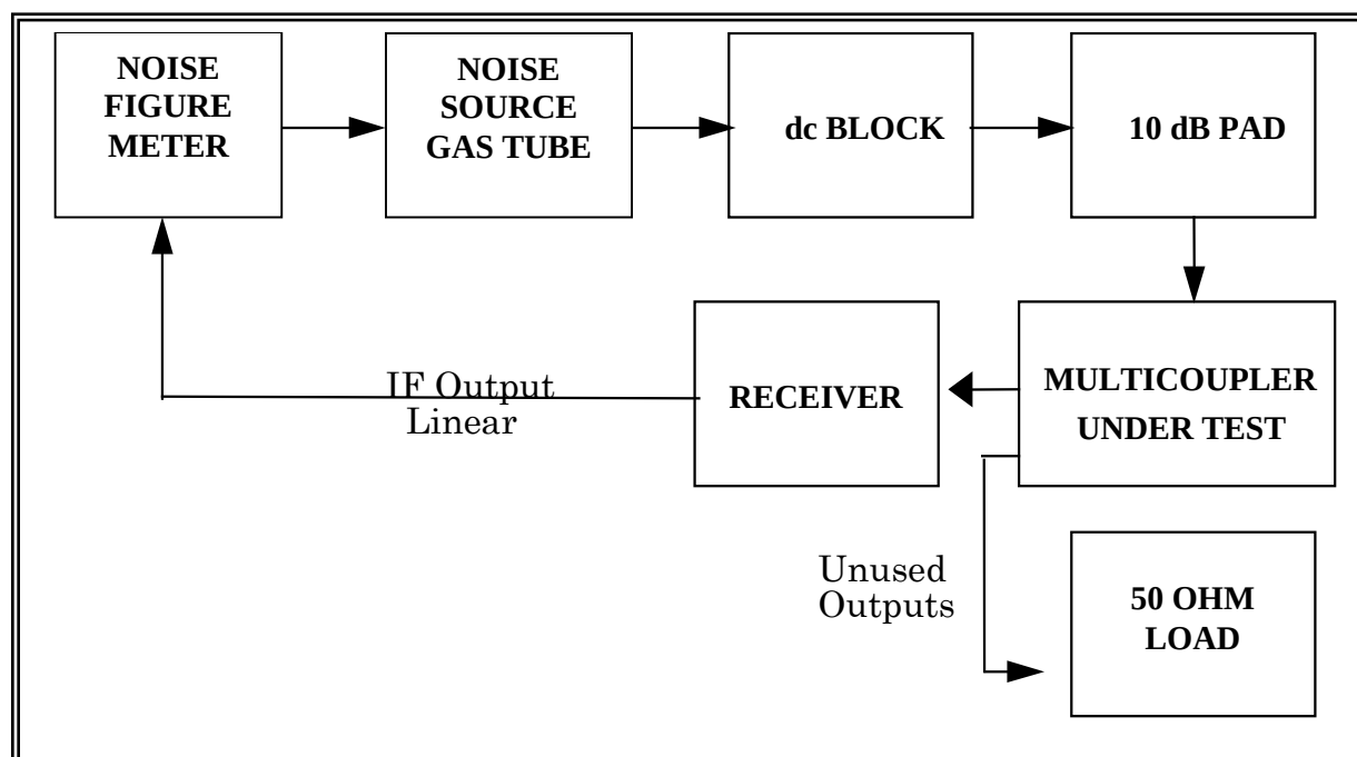
Figure 3-10a. Test setup for measurement of noise figure (see test 3.5).
