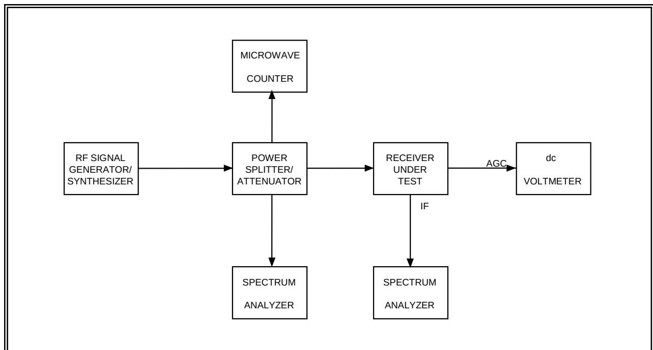
Figure 4-1. Receiver spurious signal response test (see tests 4.1 and 4.3).
