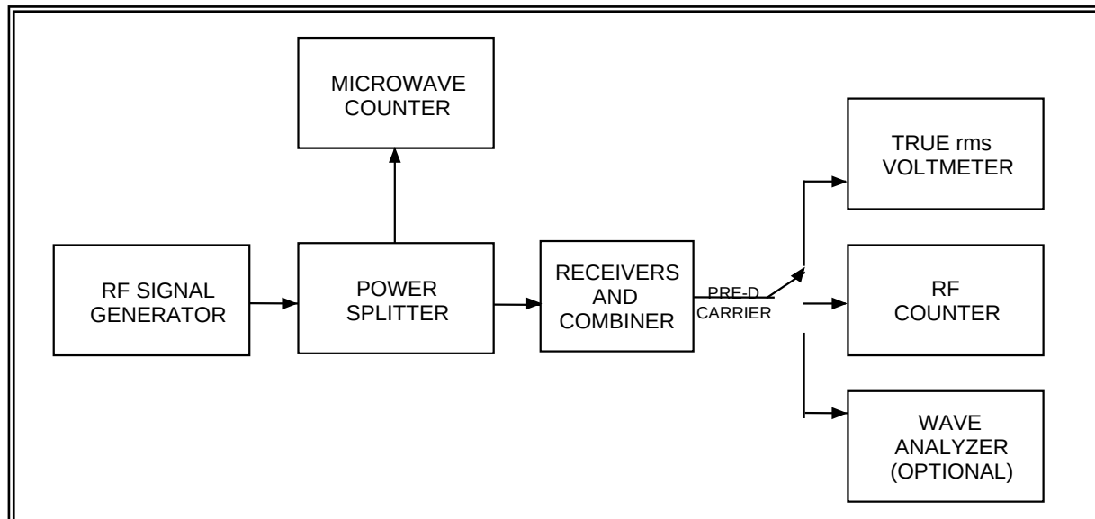
Figure 5-8. Combiner predetection carrier output (see test 5.12).
