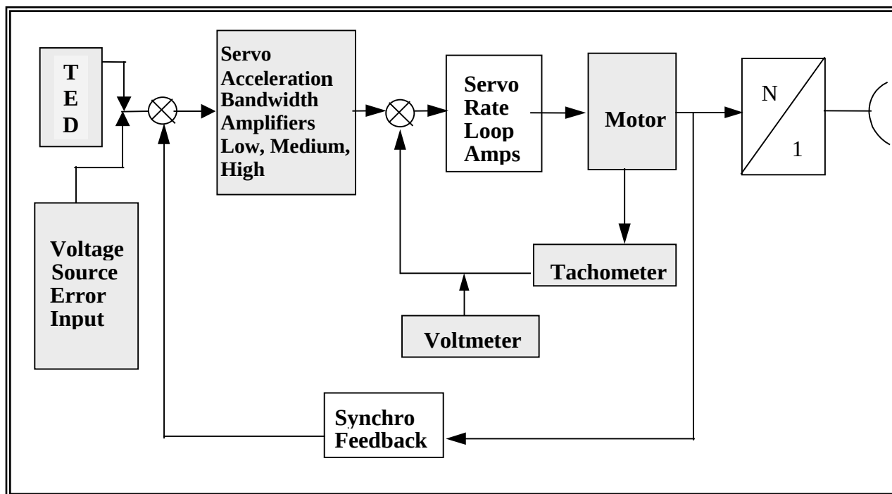
Figure 1-3. Position loop servo test block diagram (see test 1.3).
