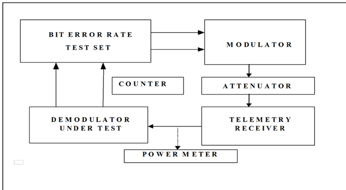
Figure 7-2. Alternate setup for demodulator bit error probability test.
