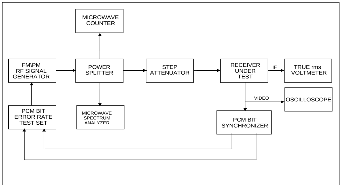
Figure 4-13. Receiver PCM bit error rate (see test 4.11).
