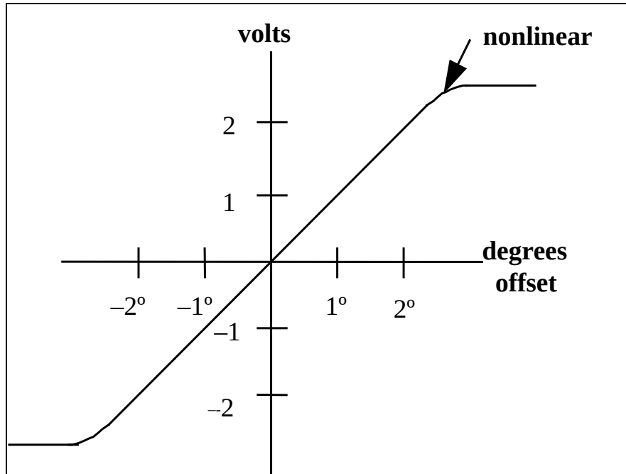
Figure 1-7. Tracking error gradient linearity slope for 1 Vdc/degree (see test 1.5).
