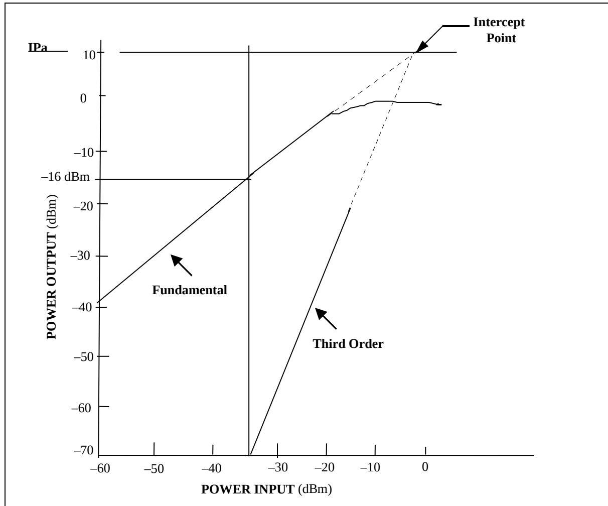
Figure 3-7. Graphical illustration of intercept point (see test 3.3).
