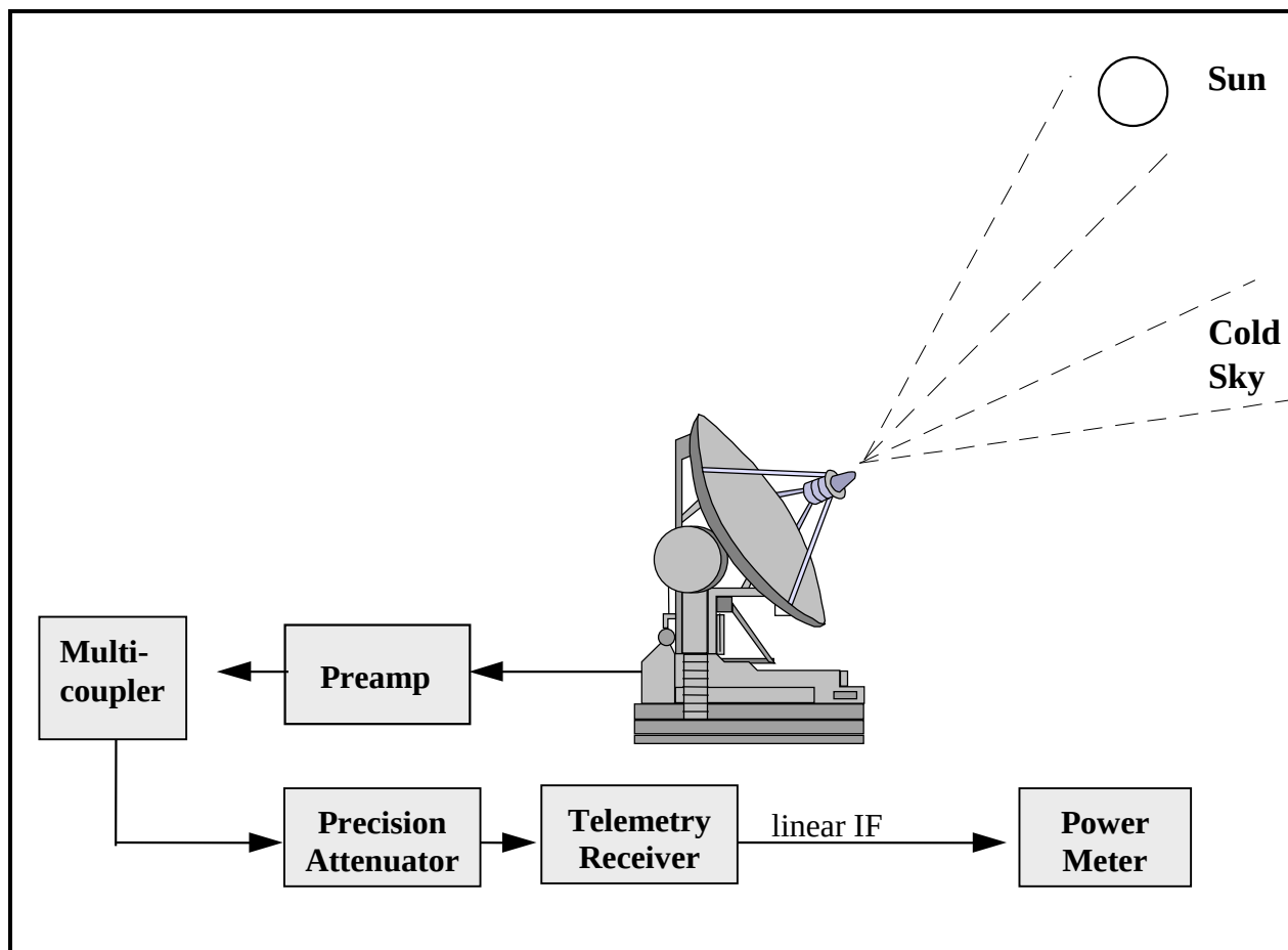
Figure 1-15. Antenna solar calibration using attenuator (see test 1.12).
