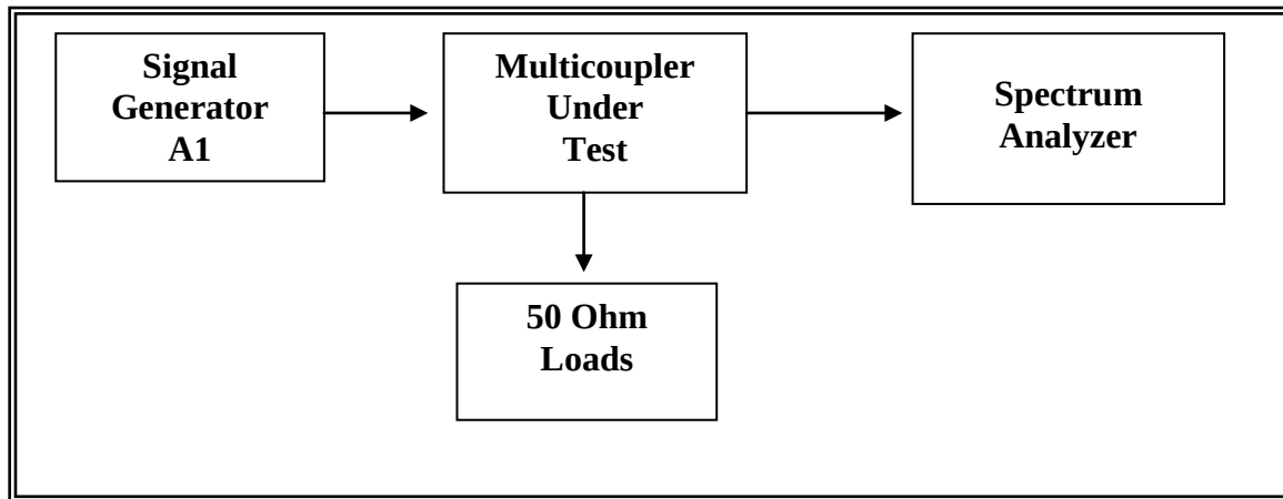
Figure 3-1. Test setup for measurement of multicoupler gain compression level (see test 3.1).
