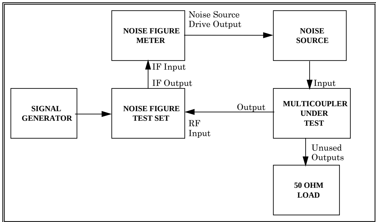
Figure 3-10b. Test setup for measurement of noise figure (see test 3.5).
