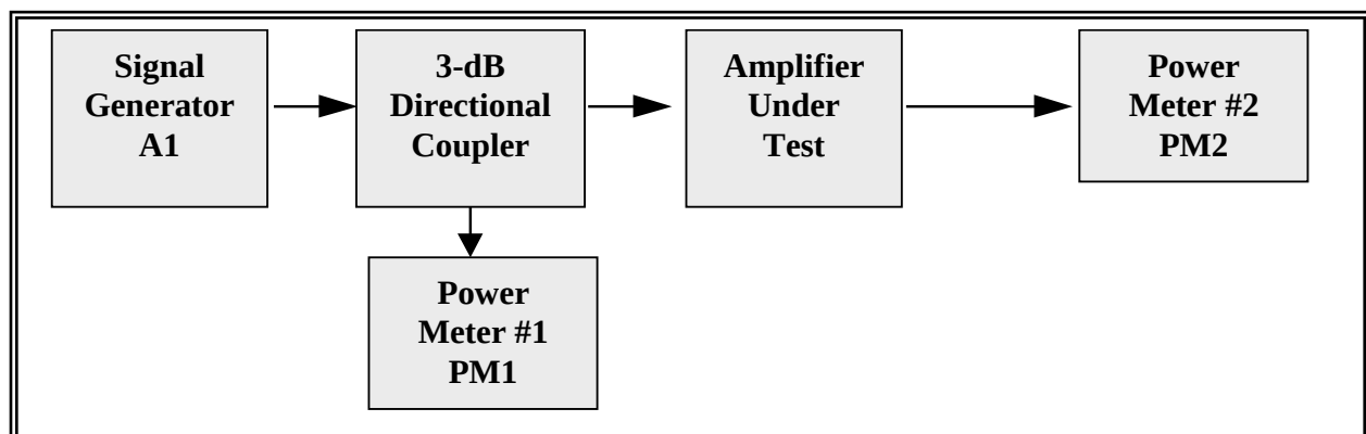
Figure 2-1. Test setup for measurement of amplifier gain compression (see test 2.1.3).
