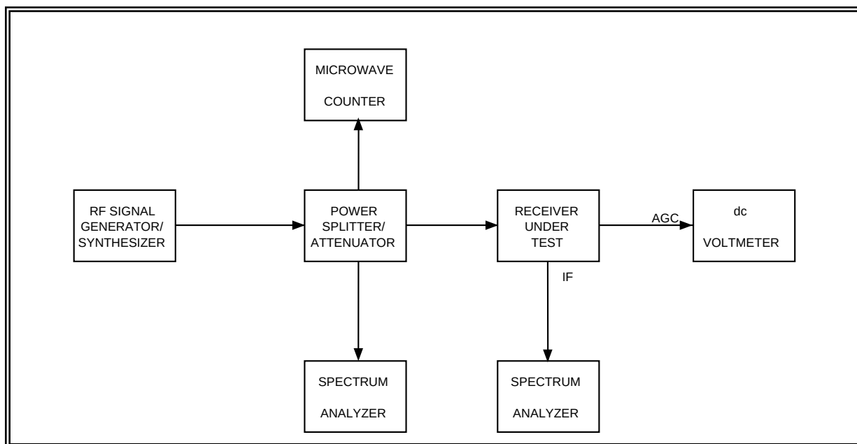
Figure 4-19. Receiver AGC stability (see test 4.17).
