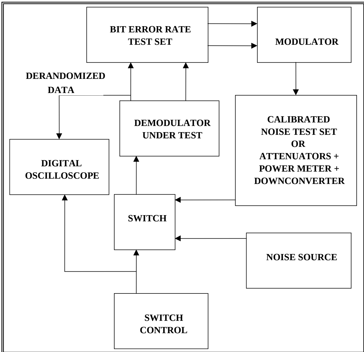
Figure 7-3. Test setup for demodulator acquisition time and flat fade recovery tests.
