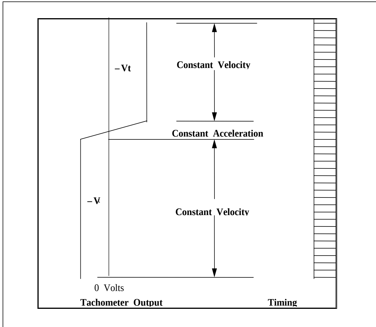
Figure 1-5. Velocity and acceleration (see test 1.4).
