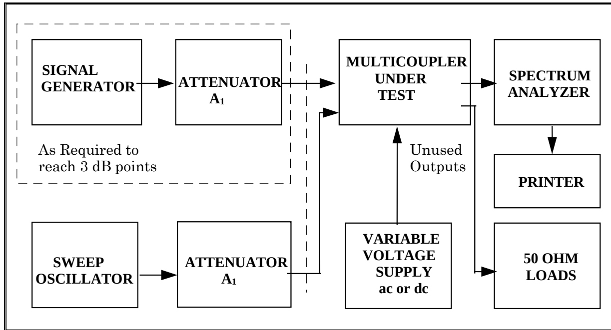
Figure 3-3. Test setup for measurement of bandwidth and small signal power gain (see test 3.2).
