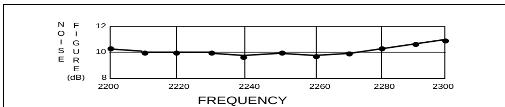
Figure 4-2. Noise figure plot (see test 4.2).
