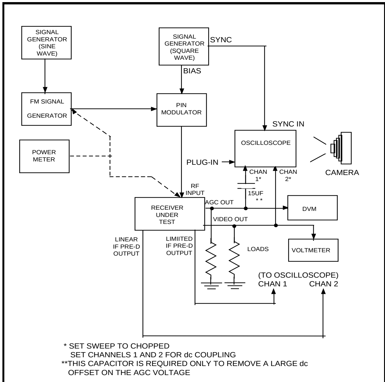
Figure 4-5. AGC response to square wave amplitude modulation (see test 4.5).
