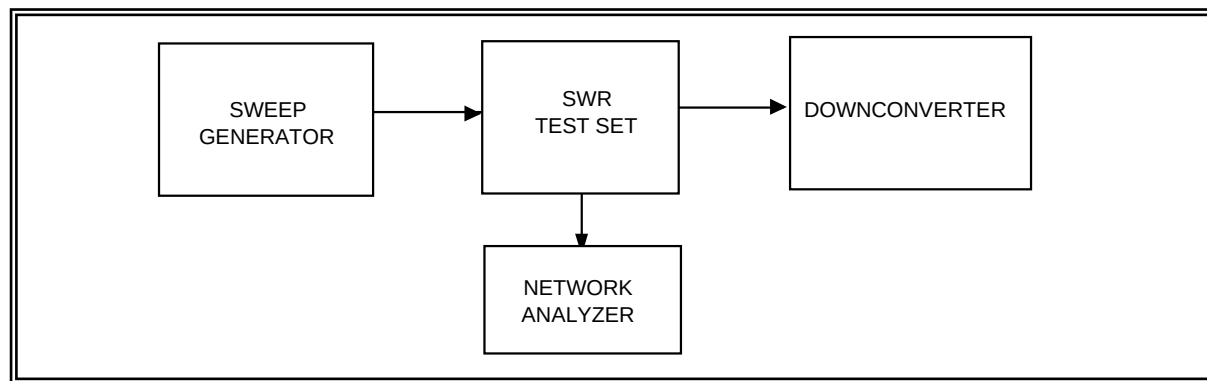
Figure 6-5. Downconverter VSWR test setup (see test 6.4).
