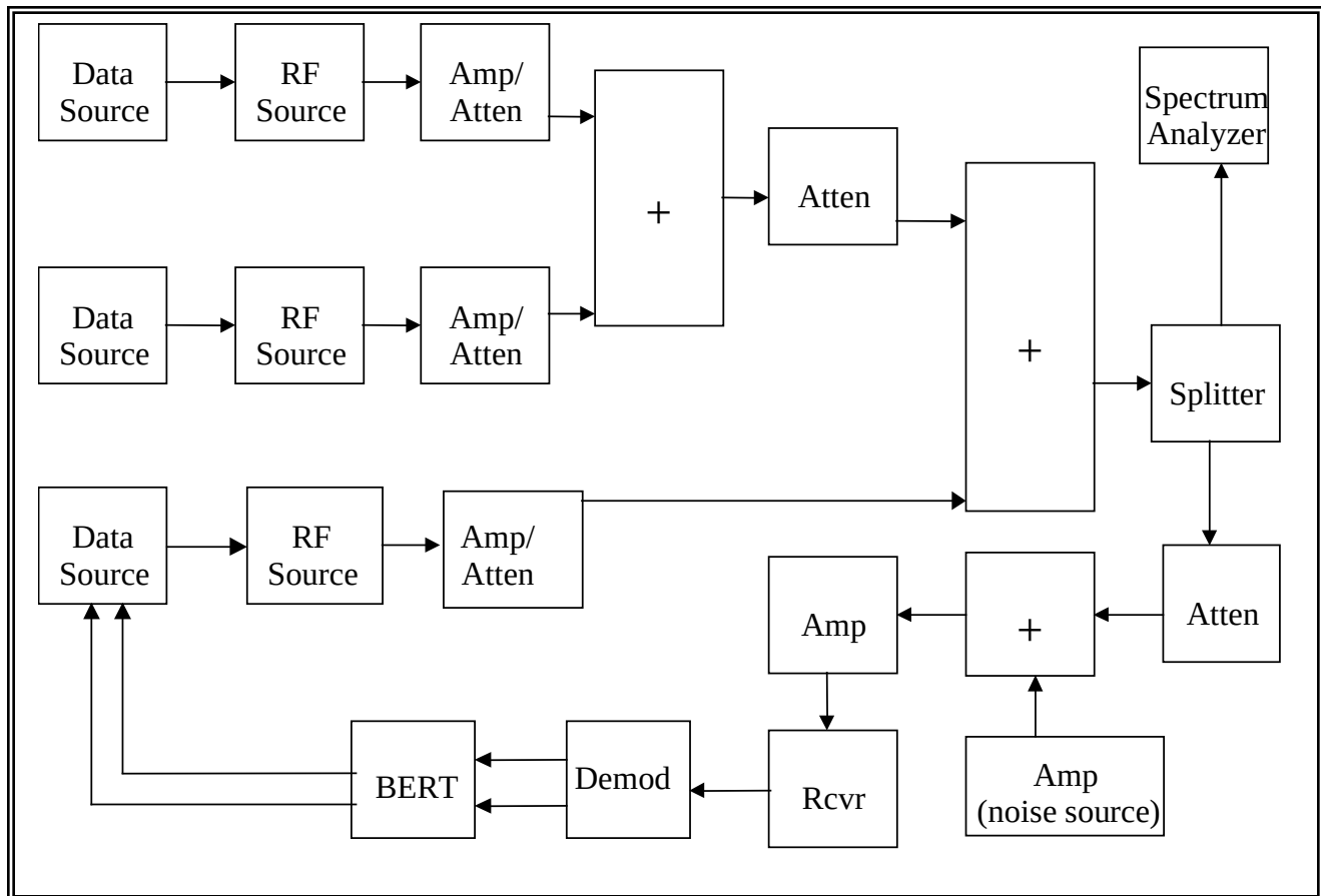
Figure 7-4. Test setup for adjacent channel interference test.
