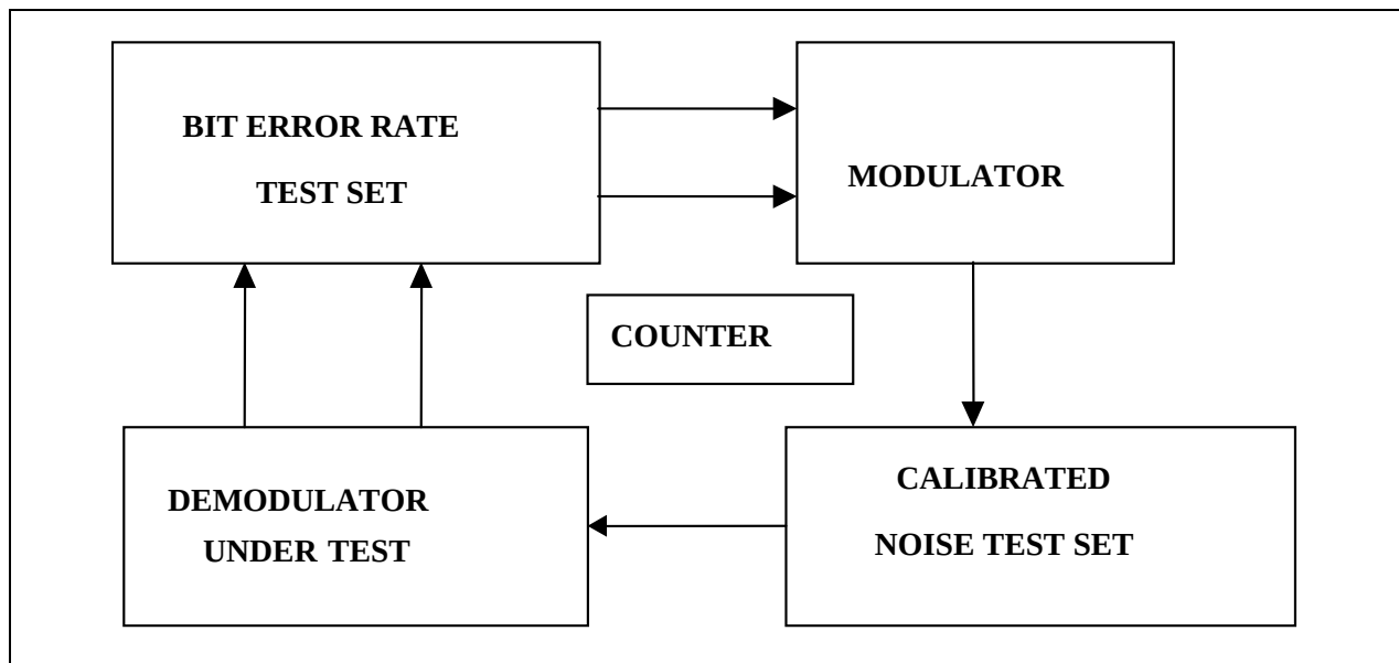
Figure 7-1. Test setup for demodulator bit error probability tests.
