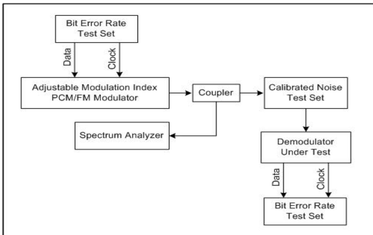
Figure 7-5. Test Setup for Modulation Index Sensitivity Test
