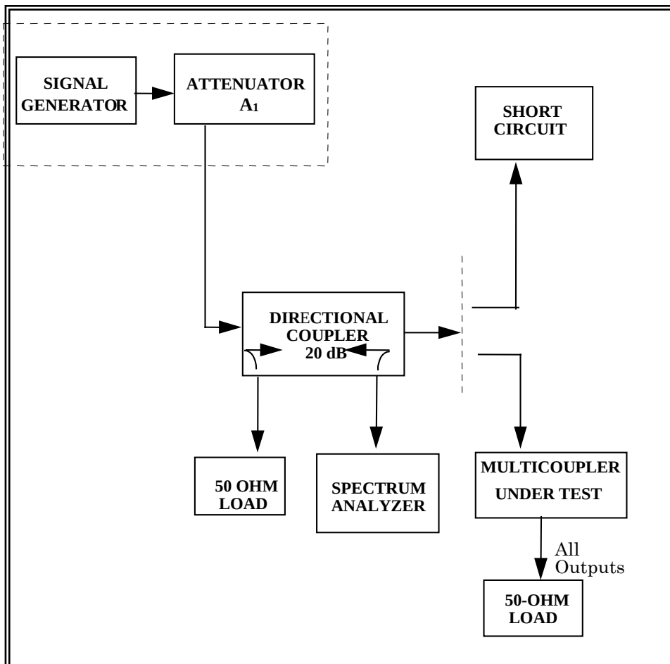
Figure 3-9b. Alternate test setup for measurement of return loss (VSWR) (see test 3.4)
