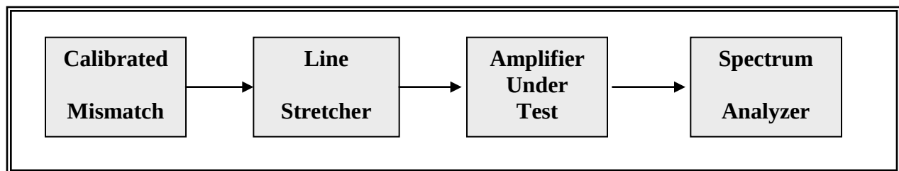
Figure 2-11. Impedance mismatch test setup (see test 2.6).
