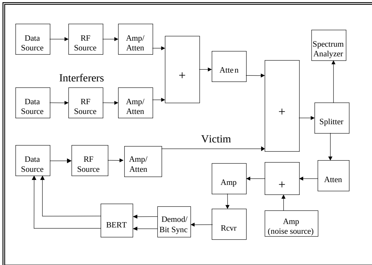
Figure 4-24. Test setup for adjacent channel interference test.
