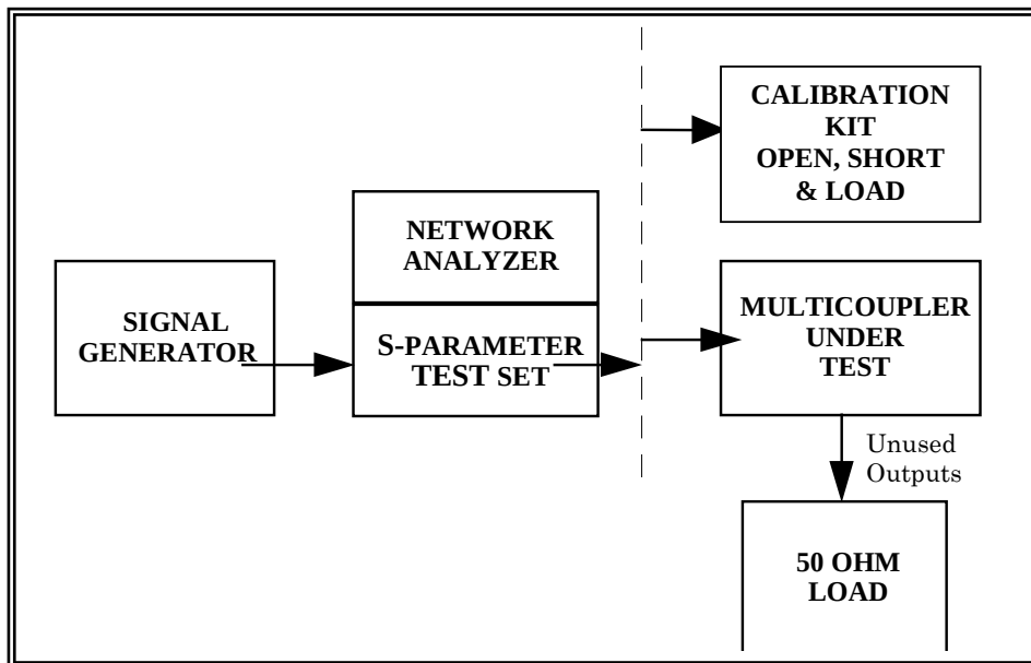
Figure 3-9a. Test setup for measurement of return loss (VSWR) (see test 3.4).
