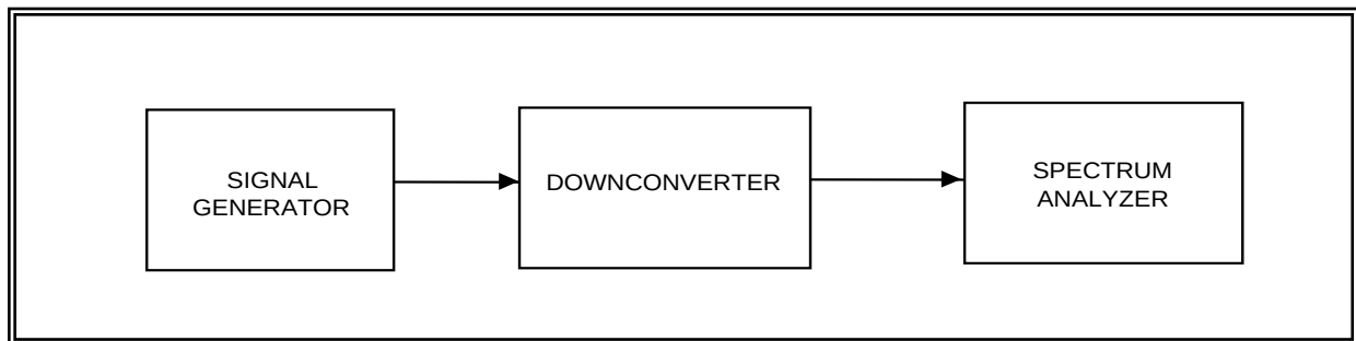
Figure 6-9. Image rejection test setup (see test 6.8).
