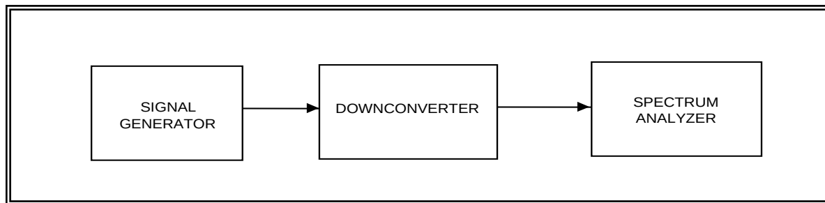
Figure 6-8. Downconverter spurious signal generation (see test 6.7).
