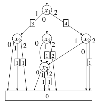
Figure 2. EVMDD for the structure function [15].
