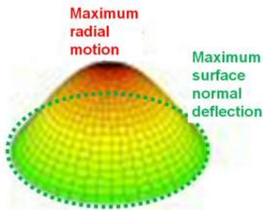
Figure 9. Circular membrane 0,1 mode vibration
