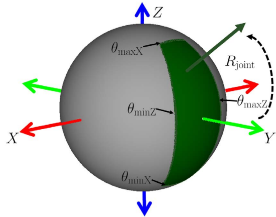
Figure 5.7: Illustration of a constrained region for a skeleton joint. The bone out of a joint is always aligned with the y-axis in the original template pose. The green region shows valid new positions into which \mathbf{R}_{\text{joint}} can rotate the bone. The four sides of the valid region are constrained by the rotation limits around the x and z -axes.
