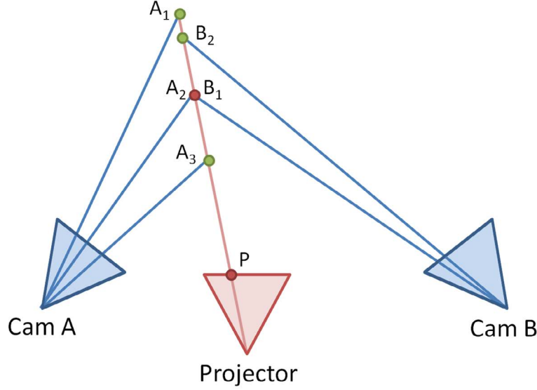
Figure 3.5: Illustration of the stereo-camera geometry used to identify correspondences across camera views.
