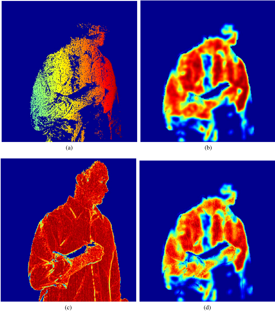
Figure 3.6: Quality map components: (a) pixels unwrapped using the approach of Sections 3.2.1 and 3.2.2; (b) density of stereo-unwrapped points; (c) local derivative measure; (d) final quality map.
