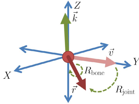
Figure 5.6: An example of the decomposition of \mathbf{R}_{\text{local}} into \mathbf{R}_{\text{joint}} and \mathbf{R}_{\text{bone}} . The original pose of a bone in P_0 always lies along the y-axis with unit vector \vec{v} . The axis of rotation used to rotate between \vec{v} and final bone position \vec{r} is \vec{k} .
