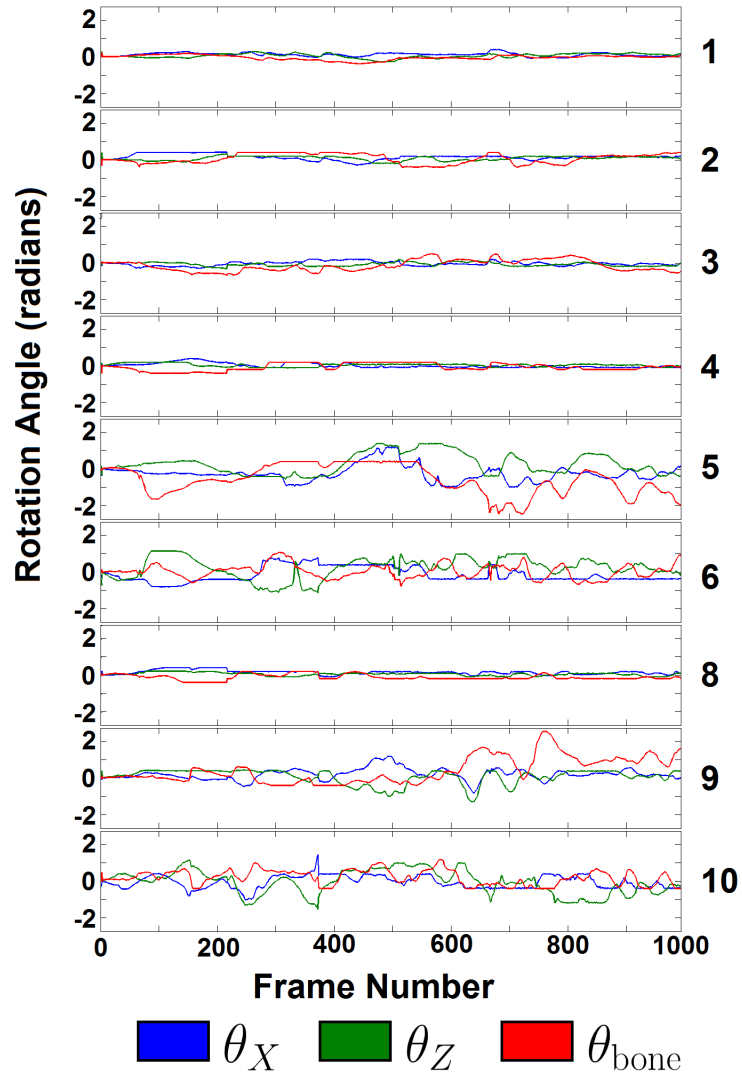
Figure 5.17: Rotation angles for branches in Fig. 5.5. For each branch, the sequence of values for \theta_X , \theta_Z , and \theta_{\text{bone}} are plotted over the frame indices.
