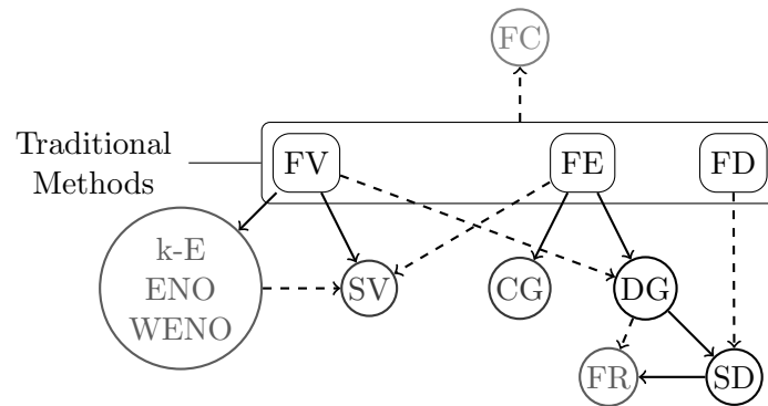
Fig. 1.1: Relationship graph for higher-order methods. The solid lines indicate a direct descent, while dashed lines indicate an indirect descent. The boldness of a method indicates its relative popularity.
