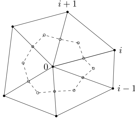
Fig. 3.2: Node-centered stencil on a two-dimensional unstructured triangular grid
