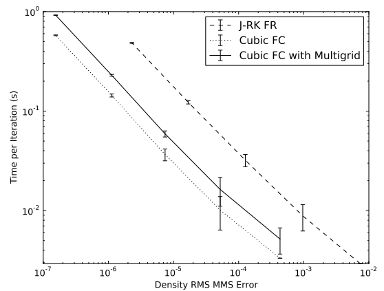
(f) FR vs FC time per iteration for given accuracy on Intel i3
