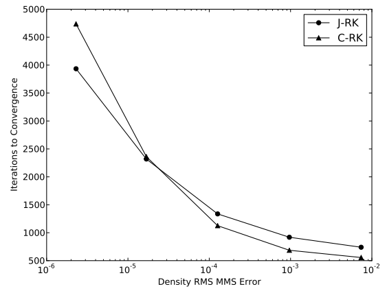
(b) FR iterations to RMS convergence for given true accuracy
