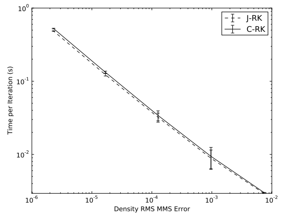
(f) FR time per iteration for given accuracy on Intel i3
