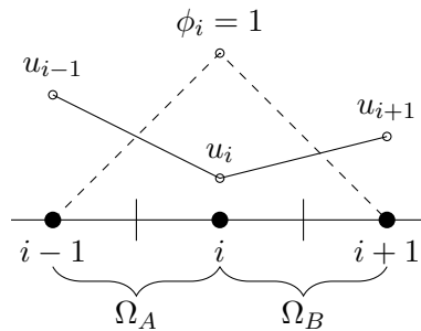
Fig. A.1: Discretization used in the derivation of the Linear Galerkin Method
