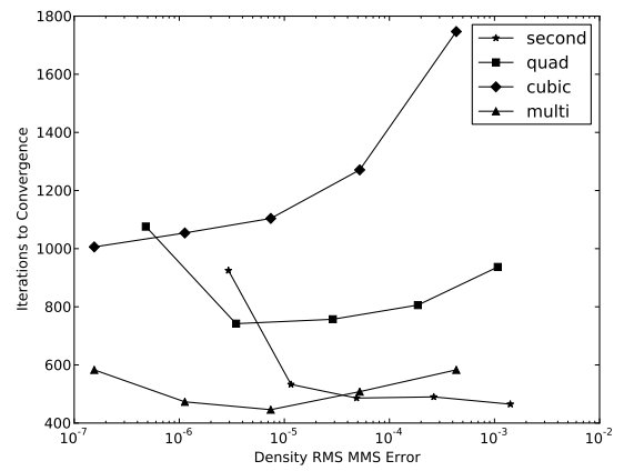
(b) FC iterations to RMS convergence for given true accuracy
