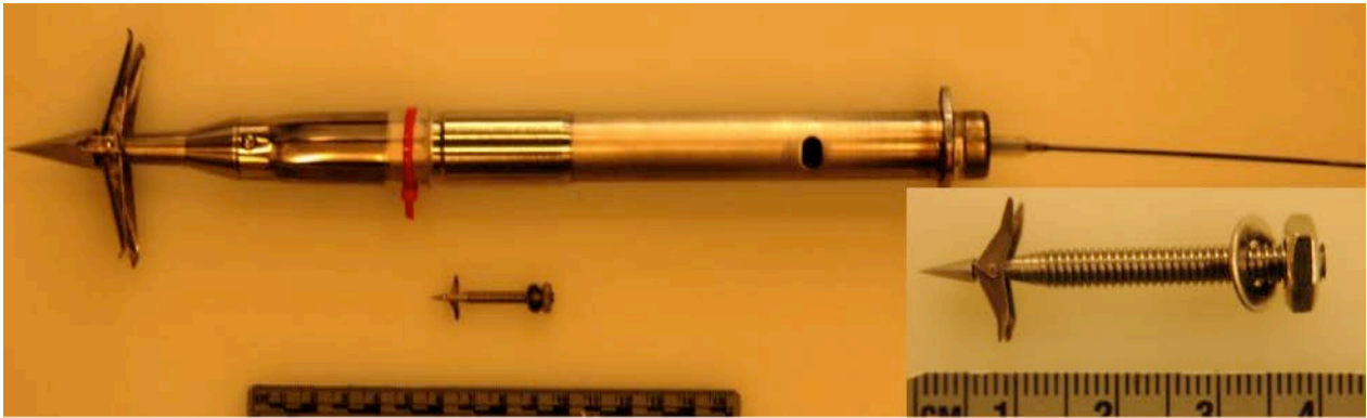
Fig. 3 – Large whale transdermal satellite tag and 1/7 th scaled dolphin dummy tag. Inset shows dummy at a larger scale. Scales in cm.
