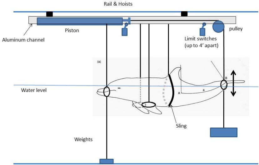
Fig. 4 – Experimental system for repeated oscillation of dolphin cadaver.
