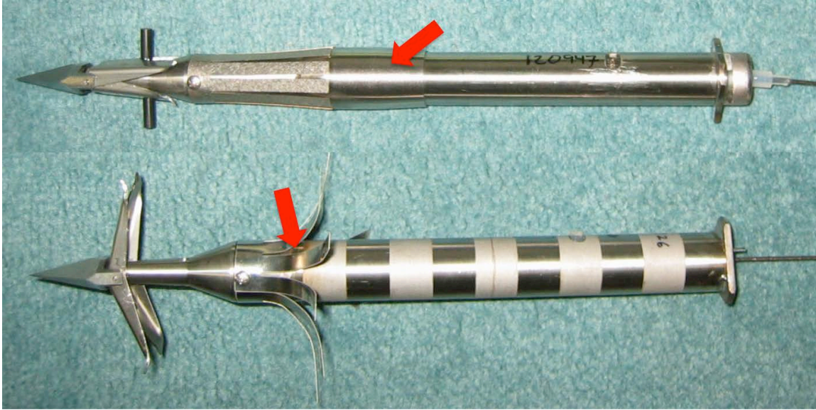
Fig. 1 – Implantable satellite transmitters showing design modifications to minimize or resolve failure of the anchor-transmitter interface. The red arrows show the reinforcement sleeve (top) created for existing tags in which welding of the transmitter body and anchor was not possible and the integrated (bottom) anchor-transmitter interface.
