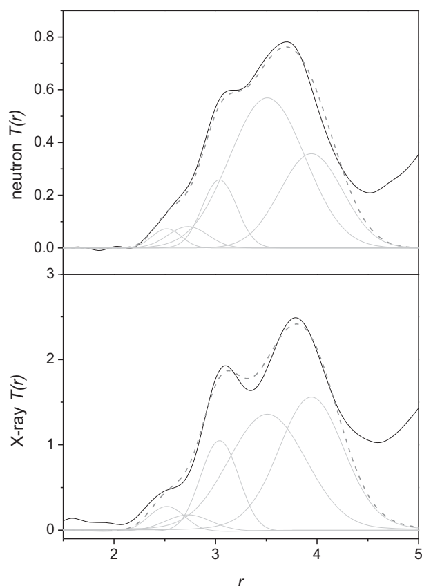
Fig. 7. Fits to X-ray and neutron correlation functions for \text{Ca}_{60}\text{Mg}_{25}\text{Cu}_{15} (the black line shows the experimental data, whilst the dashed line shows the fitted function, and the grey lines show the components of the fit).
