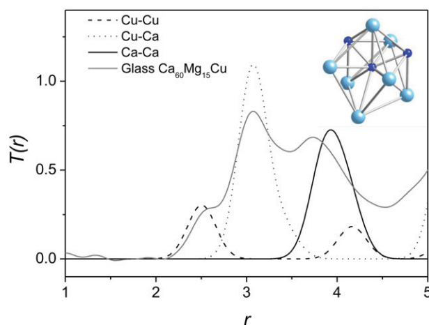
Fig. 9. A comparison the experimental T^N(r) for \text{Ca}_{60}\text{Mg}_{15}\text{Cu}_{25} with the Cu–Cu, Cu–Ca and Ca–Ca contributions simulated (see text for details) according to the \text{Ca}_2\text{Cu} crystal structure [40]. The inset shows the atomic arrangement around a Cu atom in the crystal, including all atoms closer than 3.5 Å (small spheres are Cu, large spheres are Ca).
