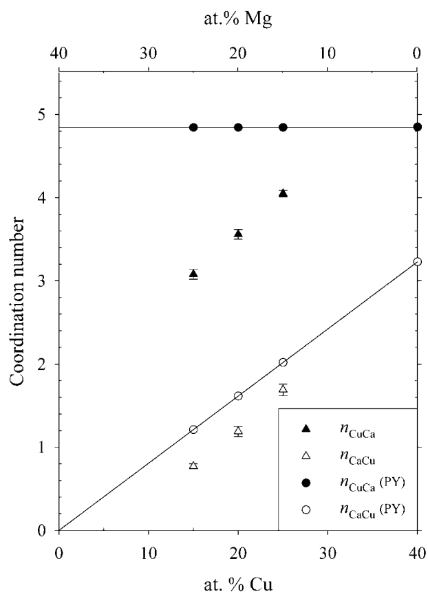
Fig. 12. n_{\text{CaCu}} and n_{\text{CuCa}} predicted on the basis of the PY simulation for \text{Ca}_{60}\text{Cu}_{40} and assuming random packing with no chemical effects (circles), together with the results from fitting the experimental data (triangles). The lines show the composition-dependence of the coordination numbers according to this approach.
