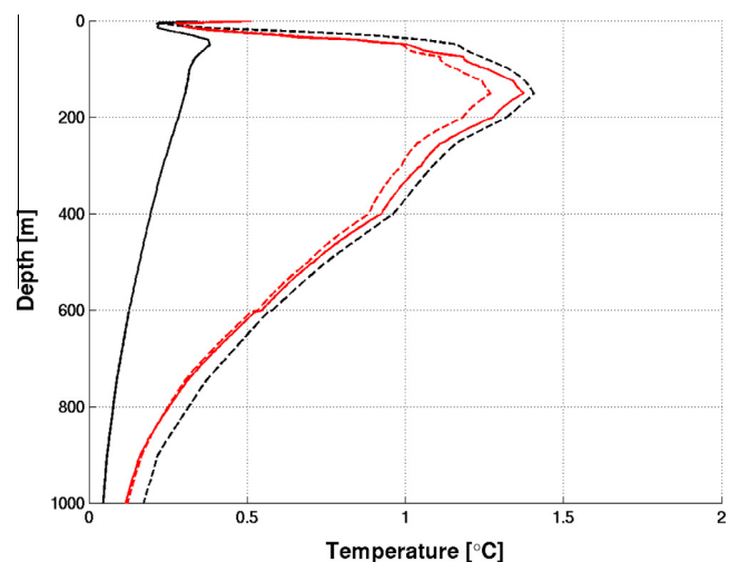
Fig. 9. Square root of the specified background error variance averaged over all observations during the experiment from R1 (solid black) and R2 (dashed black) compared to the RMS difference of observations minus background from R1 (solid red) and R2 (dashed red).
