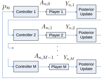
Fig. 2. Sequential scheme for M collaborative players responding to binary valued queries about the location X^* of an unknown target.
