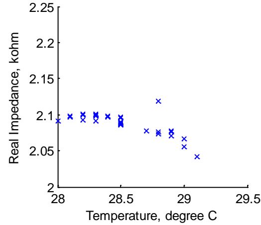
PWAS Impedance peak amplitude vs. temperature
