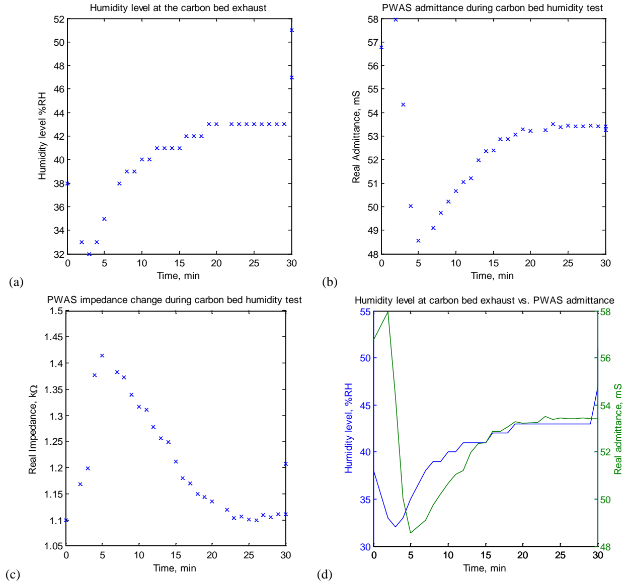
Figure 2 Experimental data from the humidity test on carbon bed embedded with PWAS. (a) Humidity level measured at the carbon bed exhaust, (b) the PWAS admittance peak value during the experiment, (c) the PWAS impedance peak value during the experiment, and (d) the comparison between the humidity level at carbon bed exhaust and the PWAS admittance peak value.
