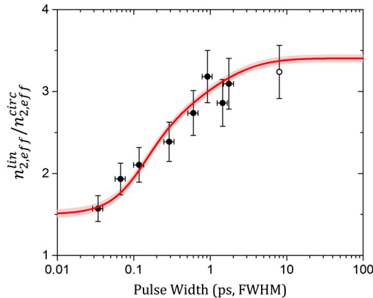
Fig. 5. Comparison of n_{2,eff}^{\text{lin}}/n_{2,eff}^{\text{circ}} versus pulse width between Z-scan measurements with both Ti:sapphire (closed circles) and Nd:YAG (open circle) laser systems at 700 nm and calculated (red curve); shaded region represents only relative errors that contribute to uncertainty.
