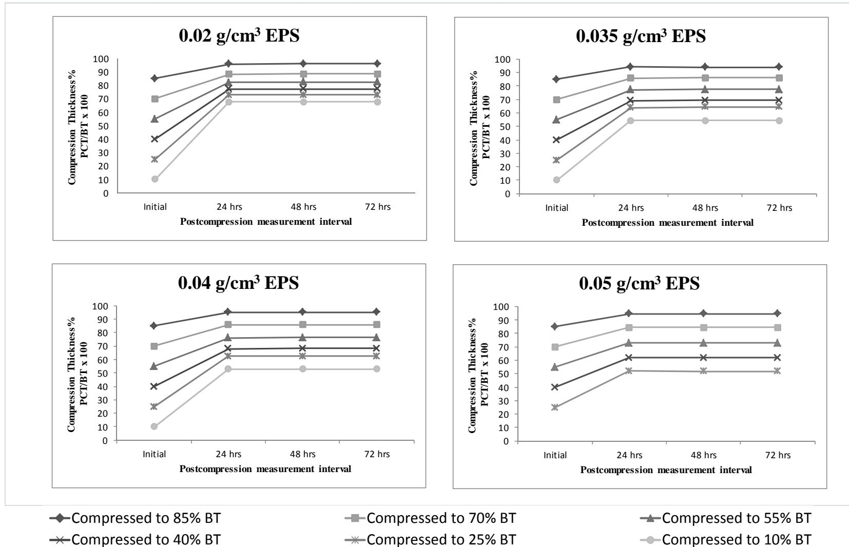
Figure 1. Mean EPS re-expansion against time. Compression of EPS of various densities and mean observed re-expansion assessed at 24-hour intervals postcompression up to 72 hours. The Instron ® 4411 material test system could not generate sufficient force to compress the 0.05 g/cm 3 EPS foam to 10 percent BT. PCT = postcompression thickness; BT = baseline thickness.
