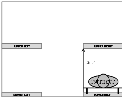
Figure 1. Scenario 1-aft view, UH-60 with IMMSS, one patient carry, treatment patient in lower right.
