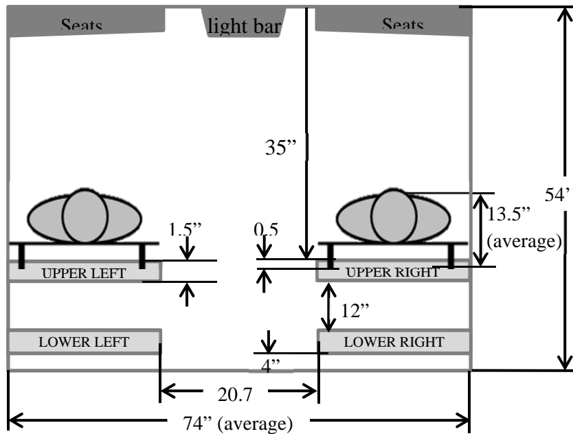
Figure A-2. Aft view – HH-60 with medical interior – SC 5 and 6 – full dimensions.
