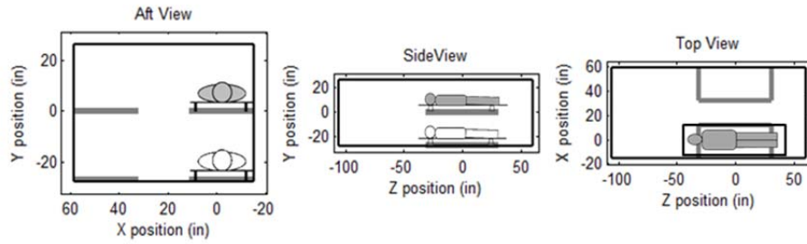
Figure C-5. Scenario 2: UH-60 with IMMUS, patient in top right litter.
