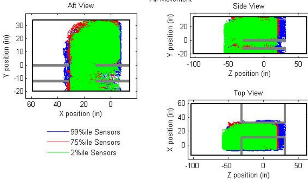
Figure C-22. Scenario 6: HH-60, patient in top right litter (all TPs, all tasks, all movements).
