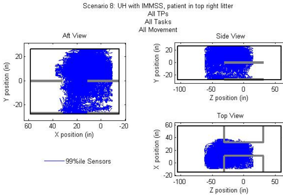
Figure C-30. Scenario 8: UH-60 with IMMSS, patient in top right litter (all TPs, all tasks, all movements).
