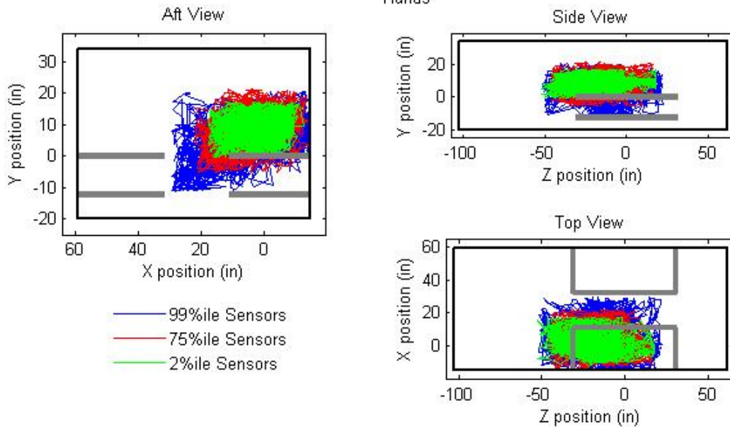
Figure C-20. Scenario 5: HH-60, patient in top right litter (all TPs, all tasks, head).
