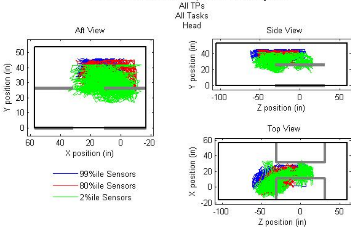
Figure C-4. Scenario 1: UH-60 with IMMSS, patient in bottom right litter (all TPs, all tasks, head).
