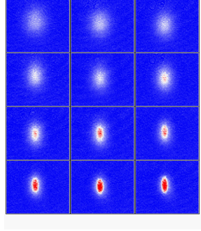
Figure 1: Formation of a Bose-Einstein condensate of {}^6\text{Li}_2 molecules in our apparatus.
