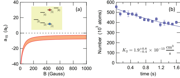
Figure 7: Stable, weakly-interacting two-state mixture of {}^6\text{Li} fermions. (a) The s -wave scattering length a_{15} for a |1\rangle - |5\rangle mixture of {}^6\text{Li} atoms as a function of field as predicted by a simple coupled channels model. The range of scattering lengths shown are for different choices of model parameters. (b) Decay of the |1\rangle - |5\rangle mixture in a gas with an initial density of 3 \times 10^{12} atoms/cm ^3 in each spin state. The decay is due to a weak dipolar loss with a measured two-body inelastic loss rate coefficient K_2 = 1.9^{+0.8}_{-0.4} \times 10^{-13} cm ^3 /s.
