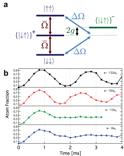
Figure 4: Observation of strong interactions producing long coherence times in a spin-1/2 Fermi gas. For sufficiently strong interactions excitation to the two-body spin-triplet state is spectroscopically resolved from excitation to the two-body spin-singlet state.
