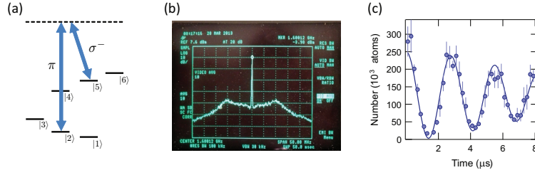
Figure 6: Two-photon Raman transition used to rapidly control interactions in {}^6\text{Li} gas by quickly switching between different two-state mixtures. (a) Two-photon Raman transition transfers population between states |2\rangle and |5\rangle . In this case, if a strongly interaction |1\rangle - |2\rangle mixture initially exists, transfer of population from state |2\rangle to state |5\rangle produces a |1\rangle - |5\rangle mixture which is weakly interacting and relatively stable against decay. (b) Beat note between two diode lasers driving the Raman transition as recorded by a spectrum analyzer. (c) Rabi oscillations between states |2\rangle and |5\rangle . The decay of contrast is due to the finite size of the Raman beams.
