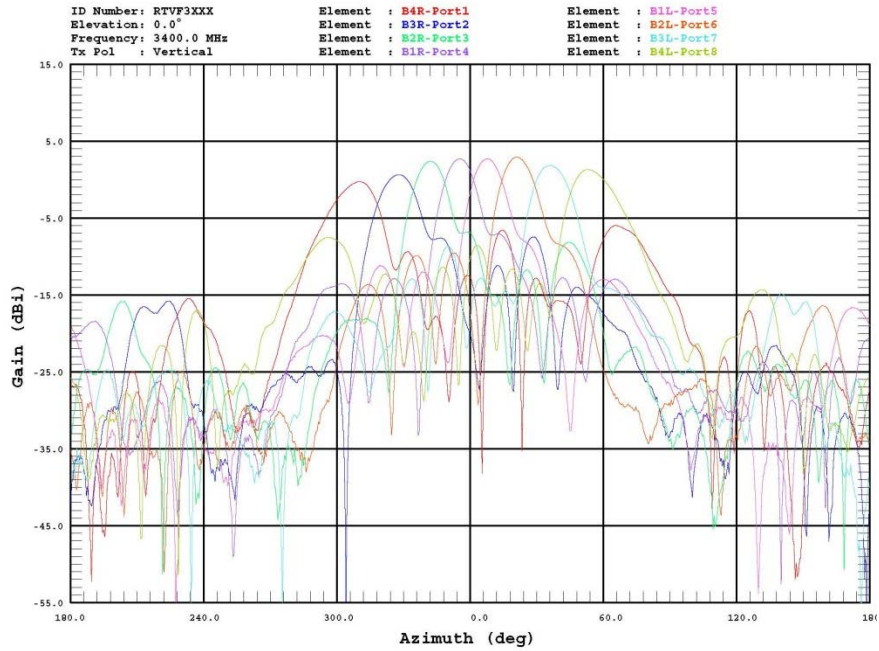
Figure 32: Eight Beam Overlay / 3400 MHz / Cartesian Plot.
