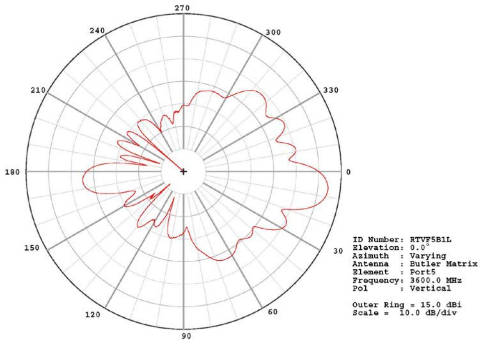
Figure 61: Beam Port 5 / 3600 MHz / Polar Plot.
