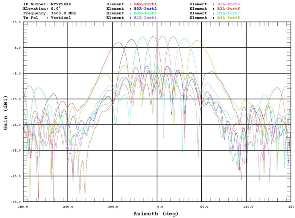
Figure 68: Eight Beam Overlay / 3600 MHz / Cartesian Plot.
