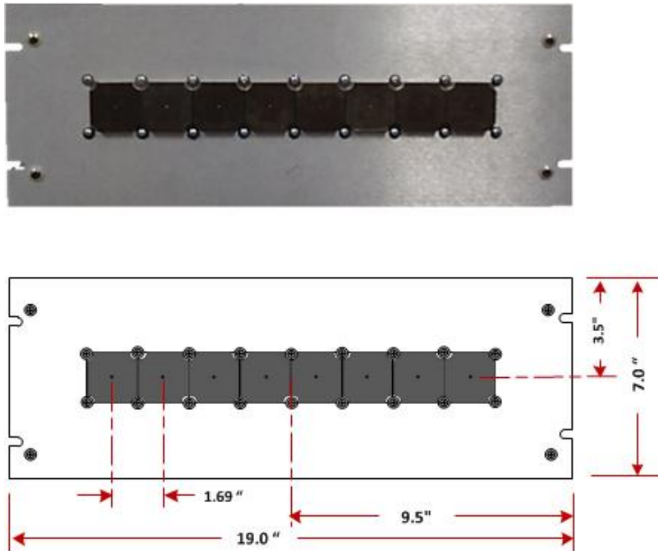
Figure 7: Array Antenna Layout.
