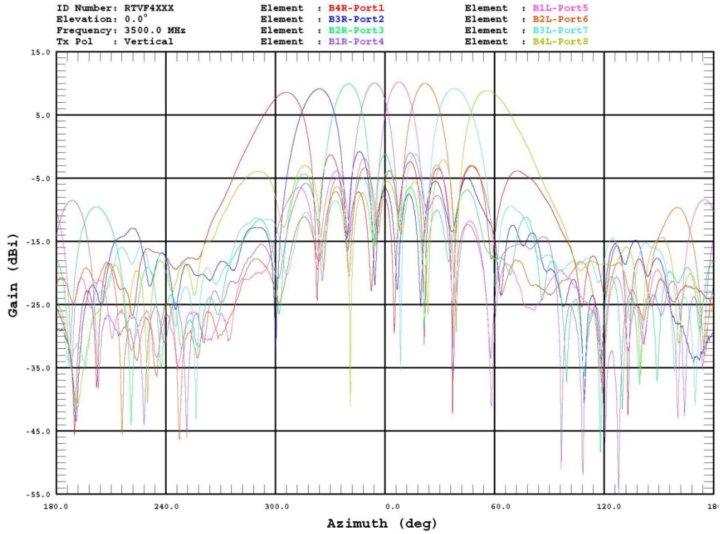
Figure 50: Eight Beam Overlay / 3500 MHz / Cartesian Plot.
