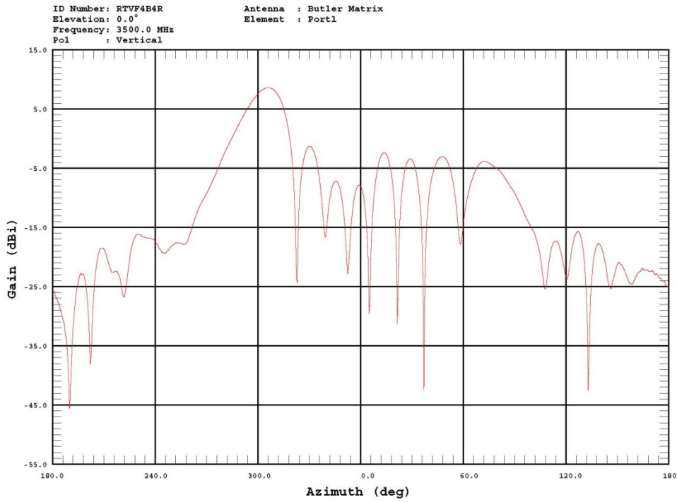
Figure 34: Beam Port 1 / 3500 MHz / Cartesian Plot.
