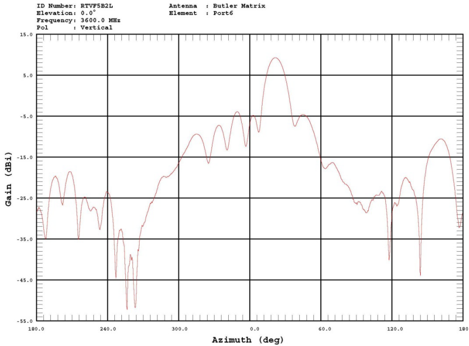
Figure 62: Beam Port 6 / 3600 MHz / Cartesian Plot.
