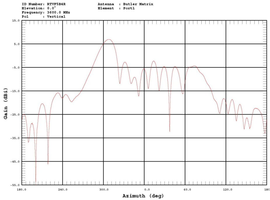
Figure 52: Beam Port 1 / 3600 MHz / Cartesian Plot.
