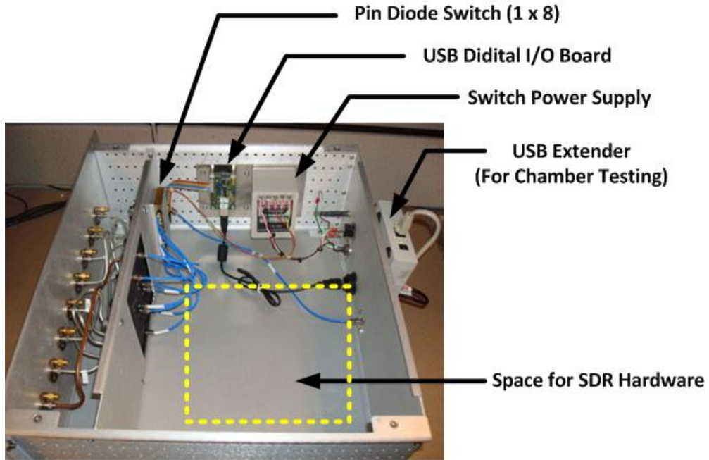
Antenna Fixture Interior
