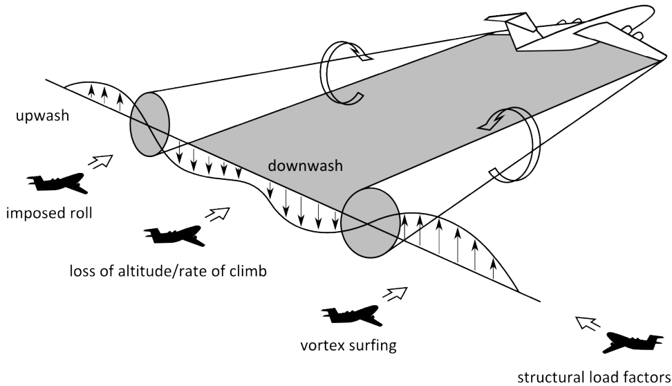
Figure 3.6. Upwash and Downwash as a Result of Lift-Induced Vortices
