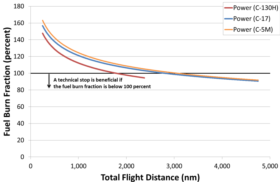
Figure 3.4. Technical Stop Fuel Burn Fraction Versus Total Flight Distance
