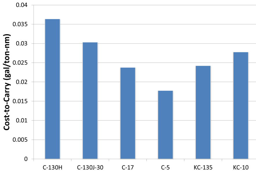
Figure 1.2. Cost-to-Carry for MAF Aircraft Across FY 2012 Flying
