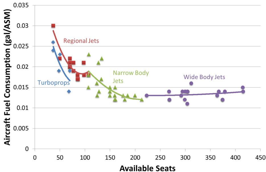
Figure 2.2. Aircraft Fuel Intensity, by Class
