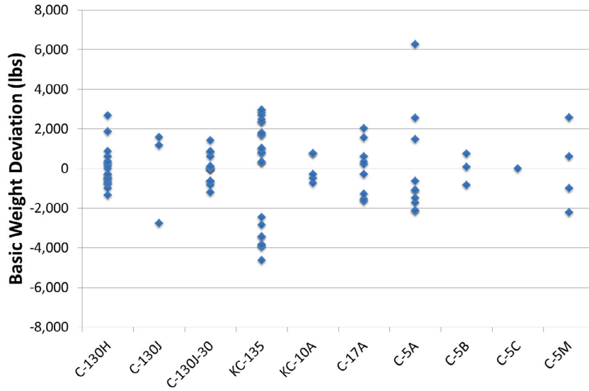
Figure 3.2. Basic Weight Deviation Between Aircraft of the Same MDS
