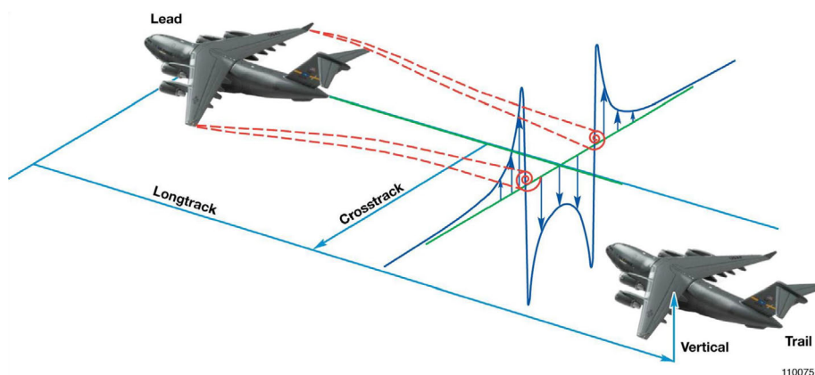
Figure S.3. Vortex Surfing Configuration
