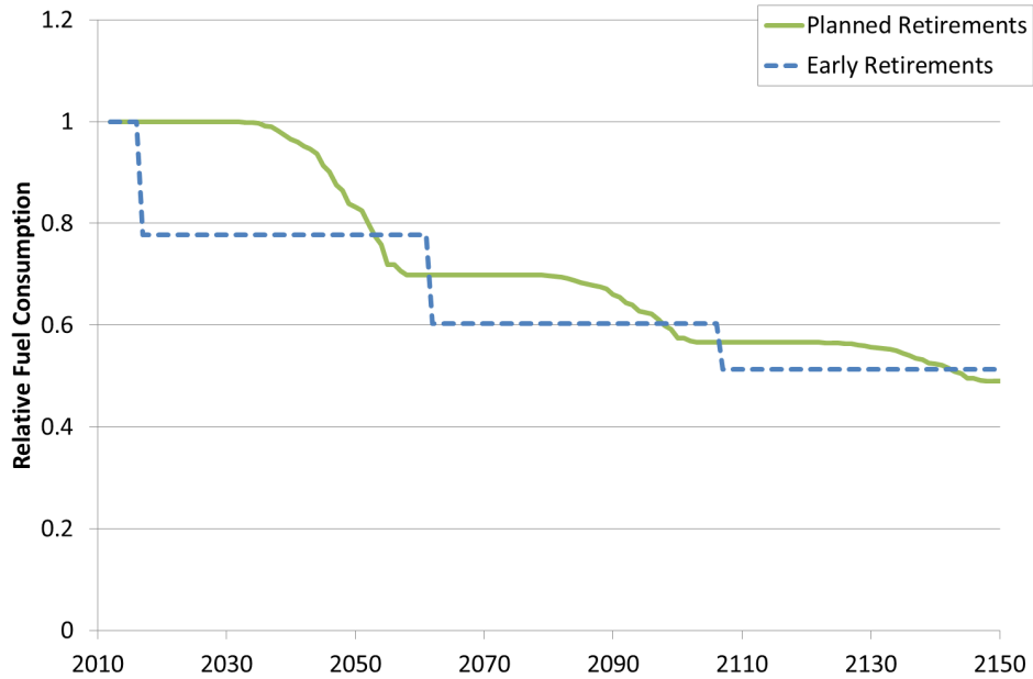
Figure 4.5. Relative C-17 Fleet Efficiency with Early Recapitalization
