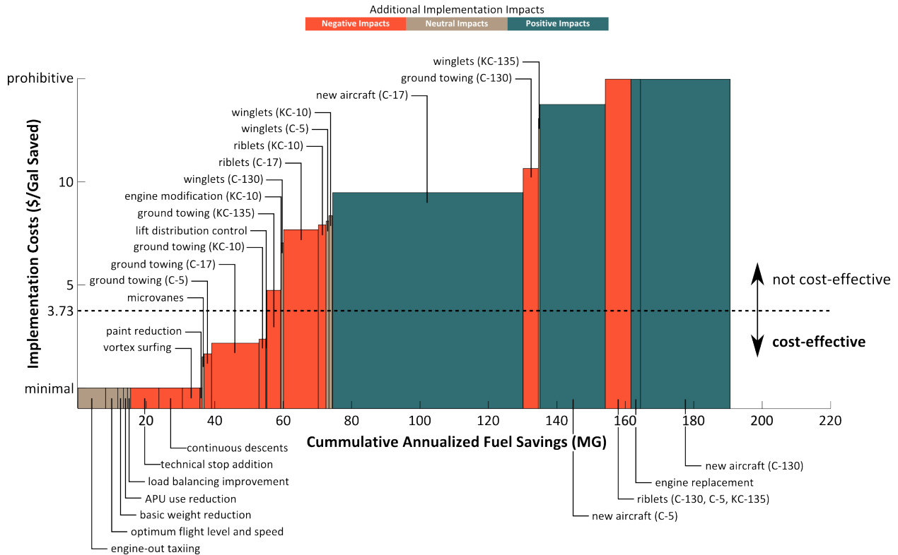
Figure S.1. Cost-Effectiveness of Fuel Reduction Options
