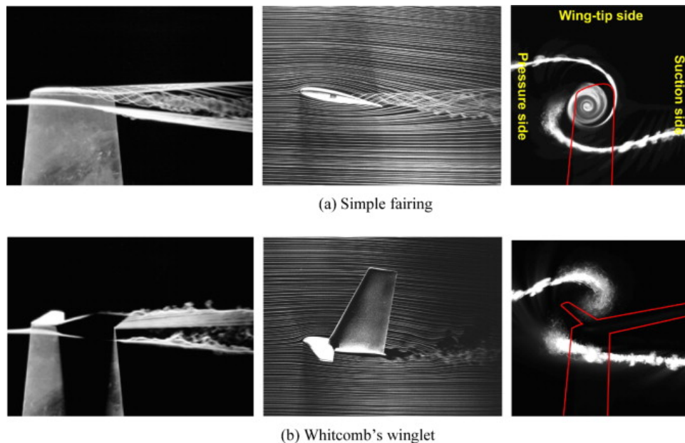
Figure 4.1. Smoke Visualization of Flow over a Simple Fairing and over Whitcomb's Winglet
