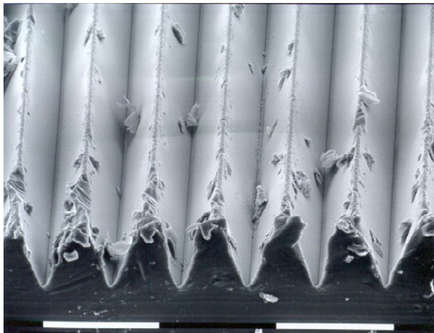
Figure 4.3. Riblets Manufactured by 3M Corporation Viewed Under an Electron Microscope
