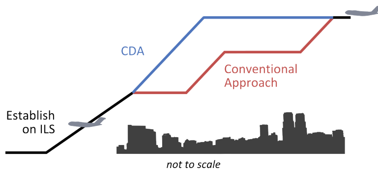
Figure 3.5. Comparison of Continuous and Conventional Descent Approaches
