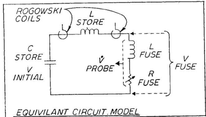
Figure 2 Test Circuit
