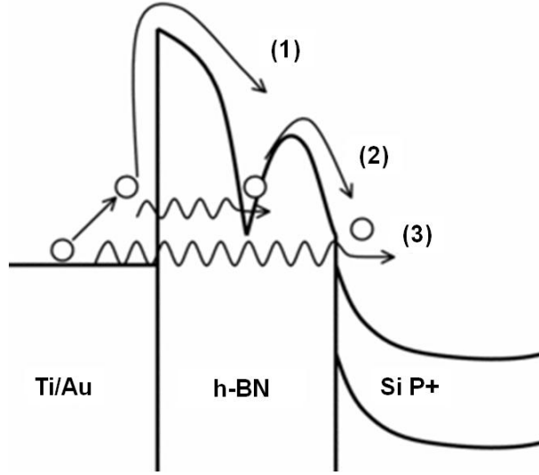
Figure 6. Energy band model of 1) Schottky emission, 2) Frenkel–Poole emission and 3) Fowler–Nordheim tunneling. Reproduced from [10].
