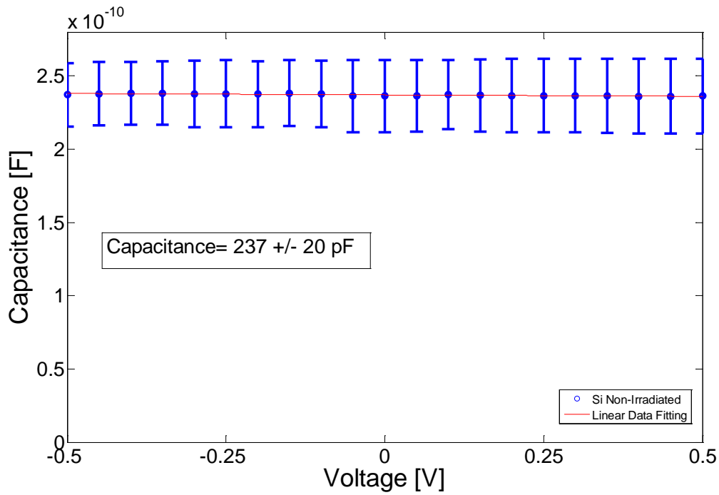
Figure 14. Capacitance as a function of voltage for p+ Si, prior to irradiation.
