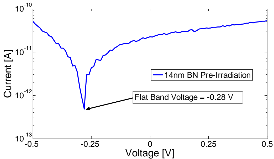
Figure 15. Current as a function of voltage for h-BN, prior to irradiation, plotted on (a) linear-linear and (b) logarithmic-linear scales.
