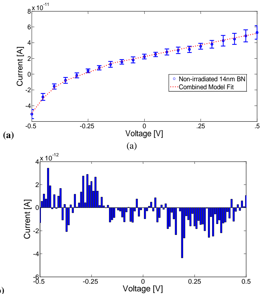
Figure 18. (a) Current as a function of voltage for 14 nm h-BN chip E, prior to irradiation, and combined FP, linear FNT, and non-linear FNT fitted models. (b) Associated residuals plot.
