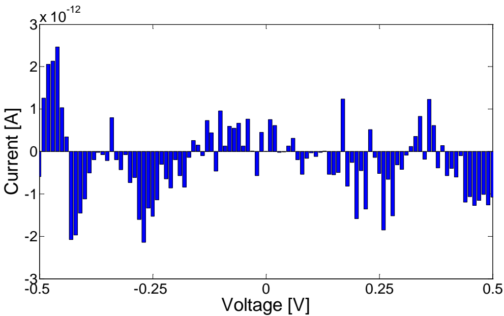
Figure 21. (a) Current as a function of voltage for h-BN chip E, with a total accumulated dose of 33.1 krad(Si), and combined FP, linear FNT, and non-linear FNT fitted models. (b) Associated residuals plot.
