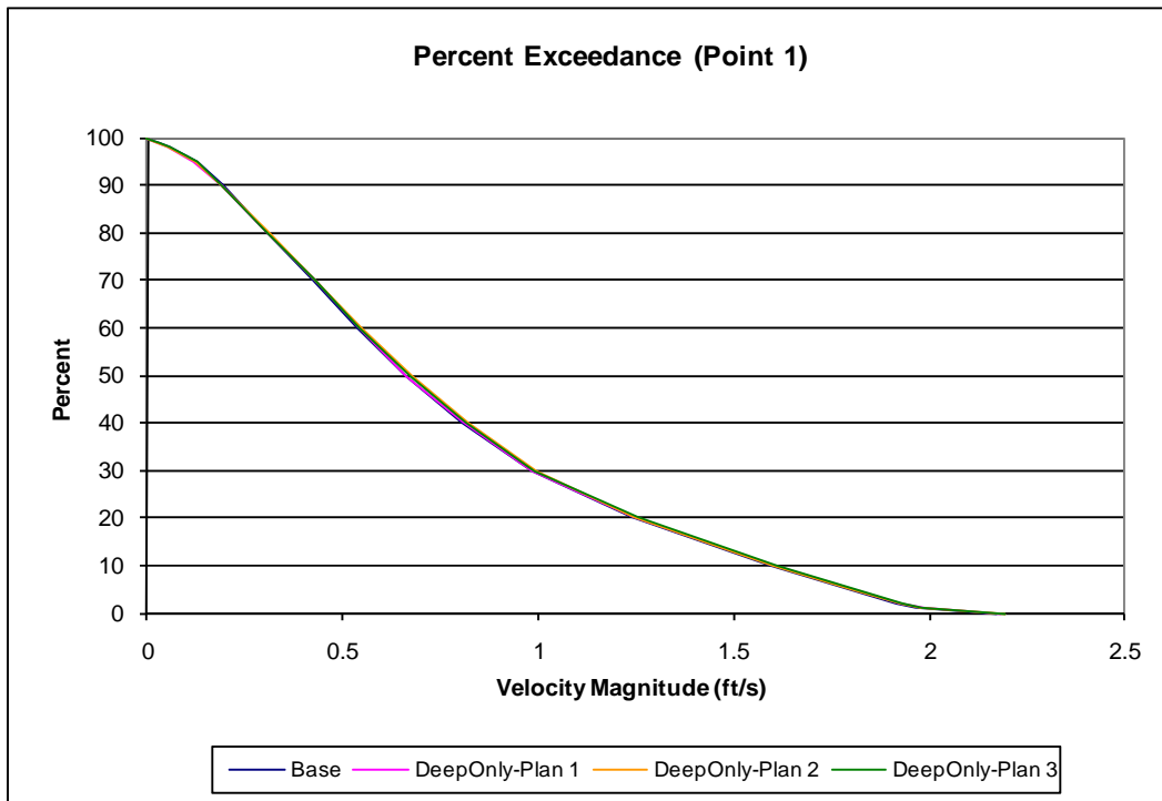
Figure 54. Percent exceedance analysis for point 1 for Deepen Only plan set.
