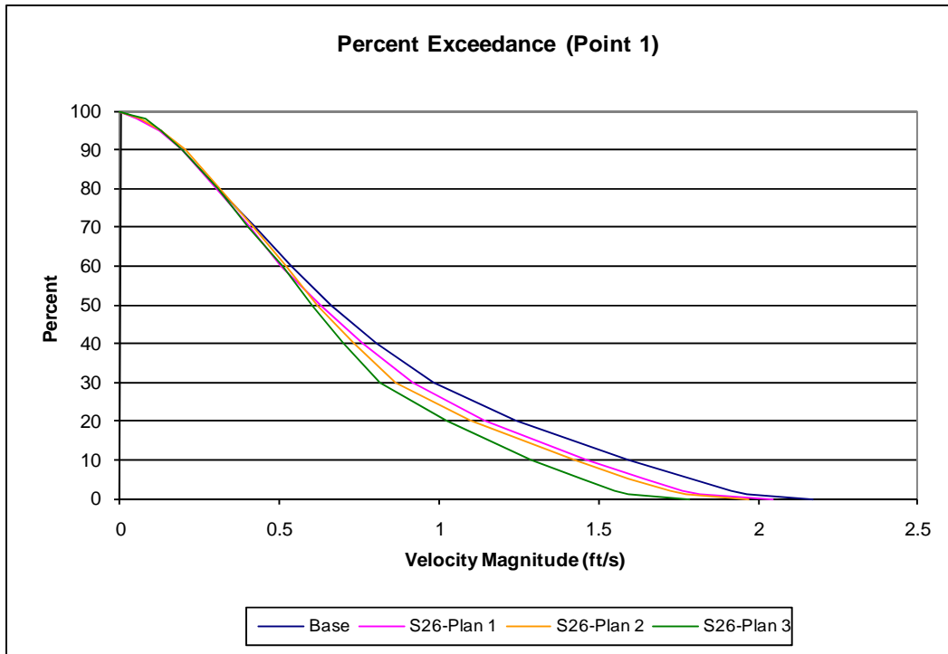
Figure 53. Percent exceedance analysis for point 1 for Station 26 plan set.
