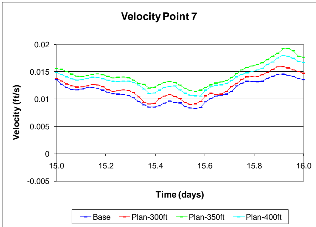
Figure 115. Velocity comparison for day 15 at point 7 for 300/350/400 plan set.
