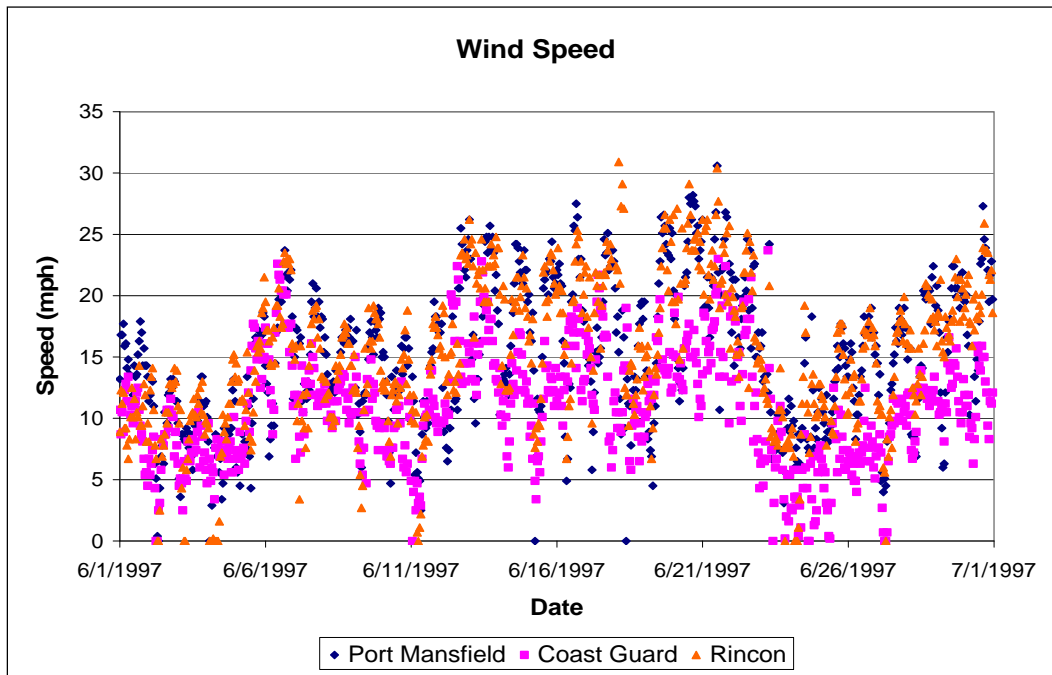
Figure 9. 1997 wind speeds.
