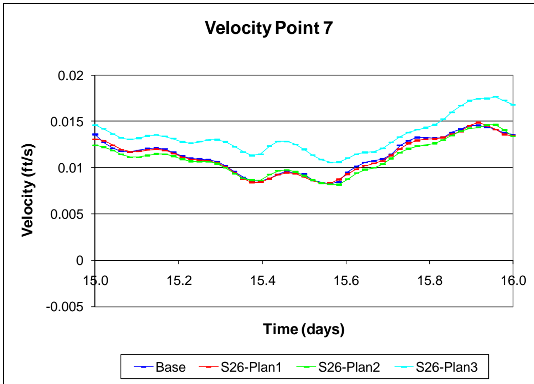
Figure 113. Velocity comparison for day 15 at point 7 for Station 26 plan set.
