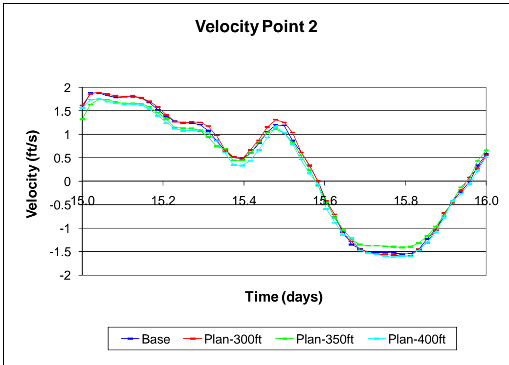
Figure 56. Velocity comparison for day 15 at point 2 for 300/350/400 plan set.
