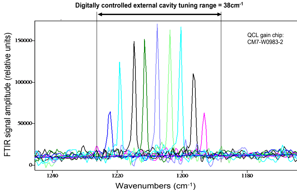
Figure 4 (a). The tuning curve for the CM7-W0983-2 chip showing tunability between 1189.7\text{cm}^{-1} and 1227.4\text{cm}^{-1} ( 8.15\mu\text{m} to 8.41\mu\text{m} ) spanning 38\text{cm}^{-1} ( 0.26\mu\text{m} ).
