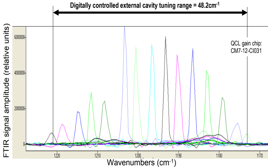
Figure 4 (b). The tuning curve of the CM7-12-CI0316 chip showing tunability between 1173.0cm -1 and 1221.2cm -1 (8.18μm to 8.52μm) spanning 48.2cm -1 (0.34μm).
