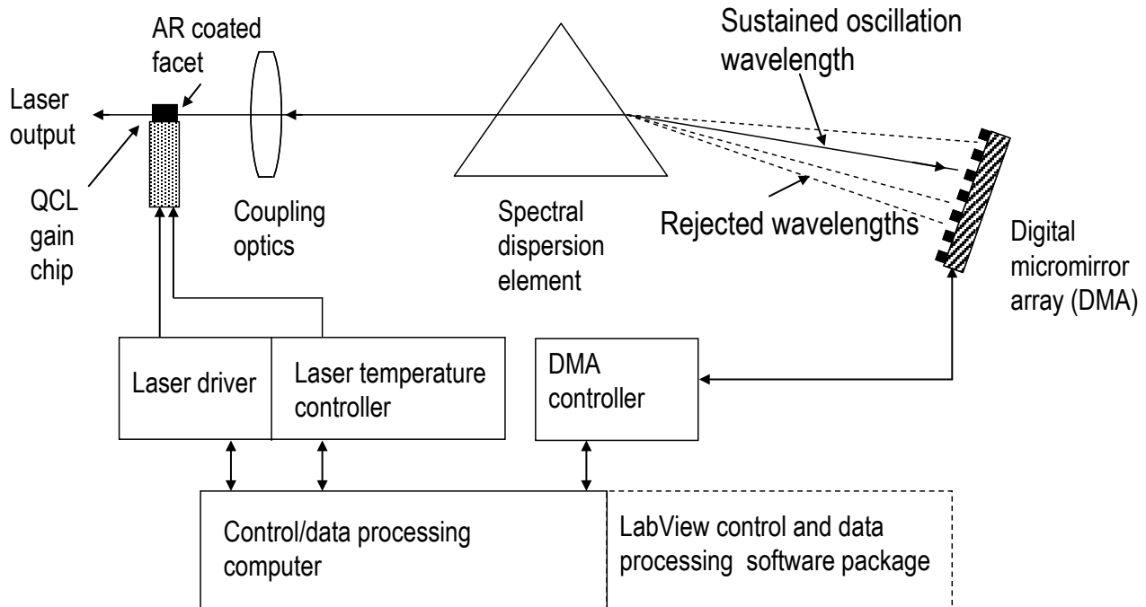
Figure 1. Digitally tunable quantum cascade laser concept.
