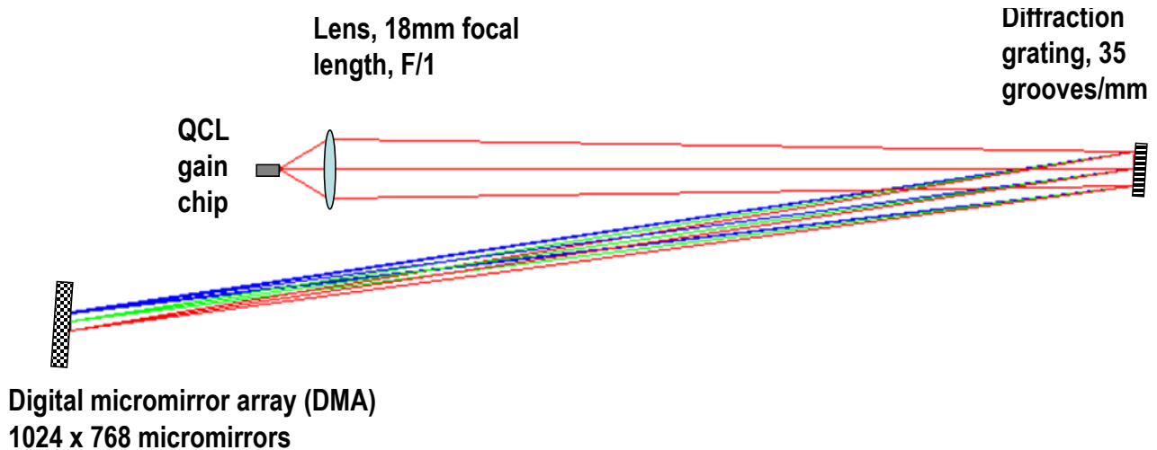
Figure 2. Tunable external laser cavity with a DMA spectral modulator.
