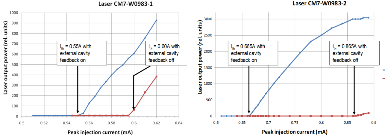
Figure 3. Laser output vs. injection current for two representative QCL gain chips, CM7-W0983-1 and CM7-W0983-2. Measured threshold currents with and without the external cavity feedback are indicated.
