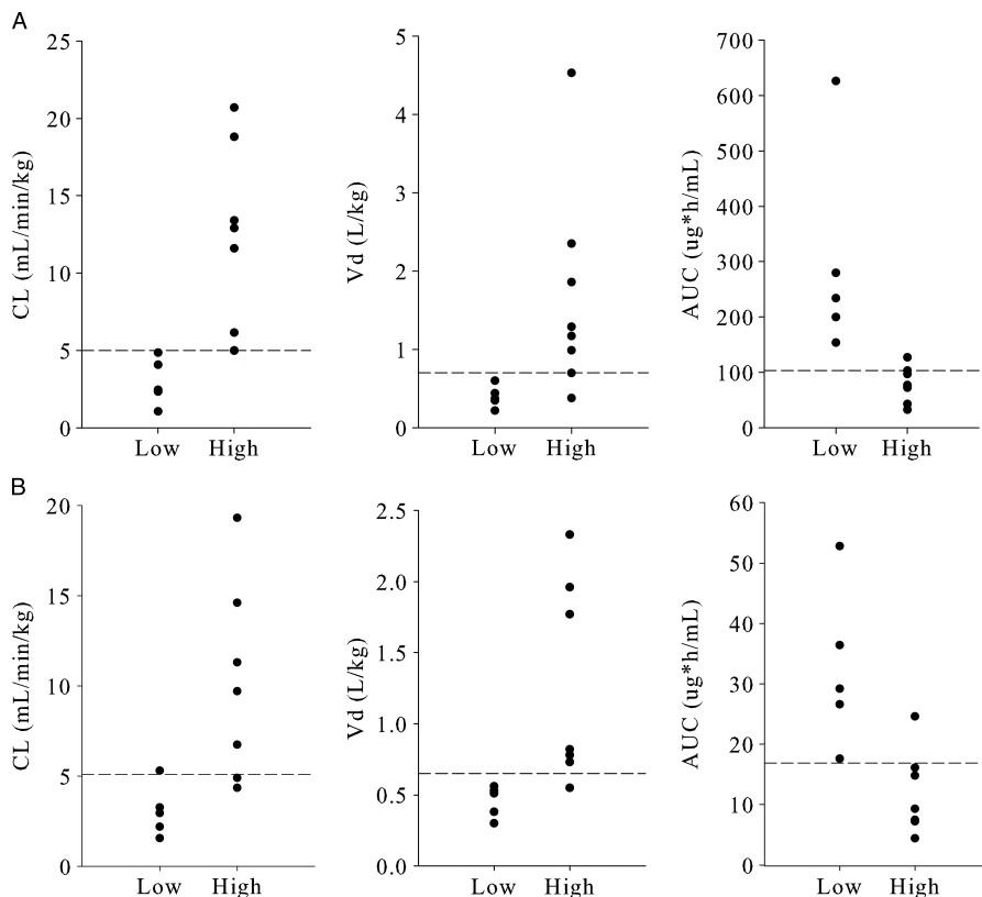
Figure 1. Clearance, volume of distribution, and AUC for free piperacillin (n = 13) (A) and free tazobactam (n = 12) (B) in patients with ARC scores of 6 or lower (low) and 7 or higher (high). Dashed line represents the population median of the low and high ARC score groups combined.
