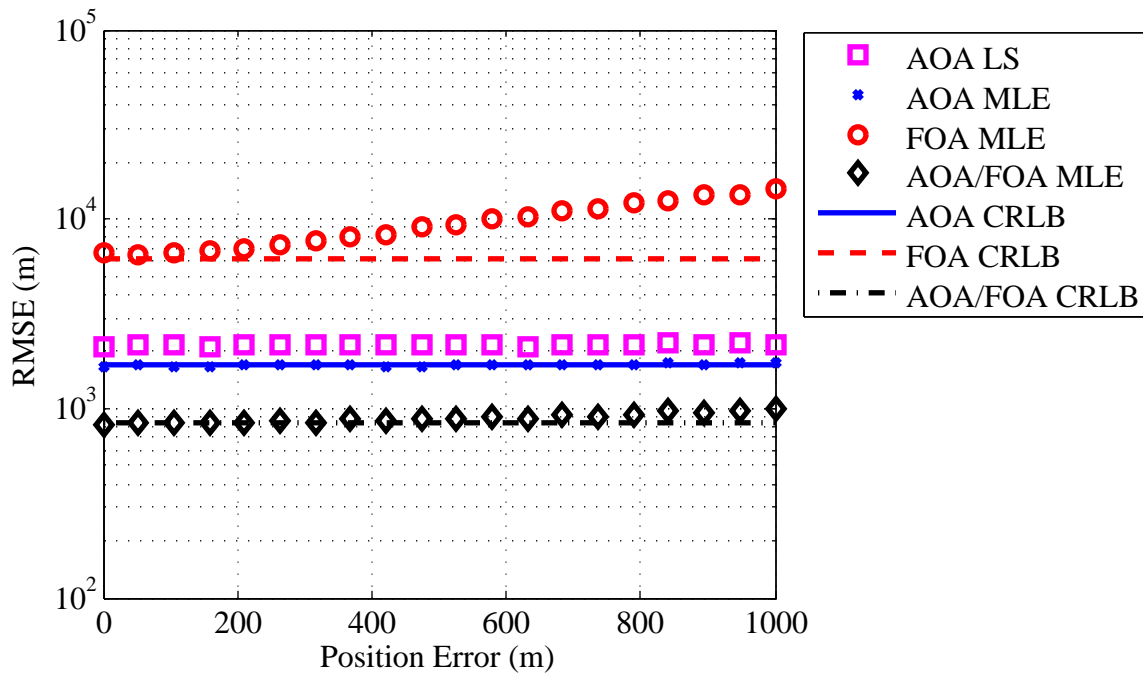
Figure 4.20: Sensitivity analysis of varying the position knowledge error standard deviation with the spinning radar emitter.
