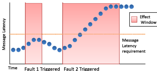
Fig. 1. Determining fault injection outcome.
