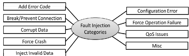
(b) Categories of injected faults derived from the fault model.
