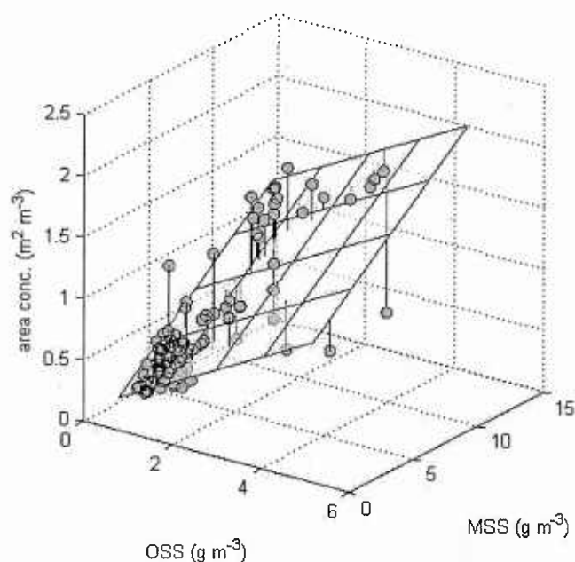
Figure 1. Area concentration in suspension versus organic suspended sediment concentration (OSS) and mineral suspended sediment concentration (MSS). Data from Dave Bowers were collected in a range of coastal environments. The plane shows the best fit linear regression of area concentration on OSS and MSS. If particle composition is uncorrelated with the packing geometry of flocs, then the ratio of the regression coefficient for OSS to the regression coefficient for MSS should be approximately equal to 2. The observed ratio is 2.12. This result suggests that compositional variability accounts only for a 2x range of variability in the c_p :SPM ratio.
