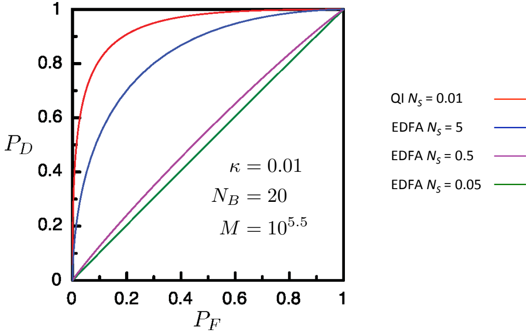
Figure 6: Receiver operating characteristic comparison between OPA reception of a quantum-illumination source and direct-detection of an EDFA source of the same bandwidth. N_S = source brightness (photons/mode); \kappa = roundtrip transmissivity; N_B = background brightness; and M = number temporal modes (EDFA) or mode pairs (QI).
