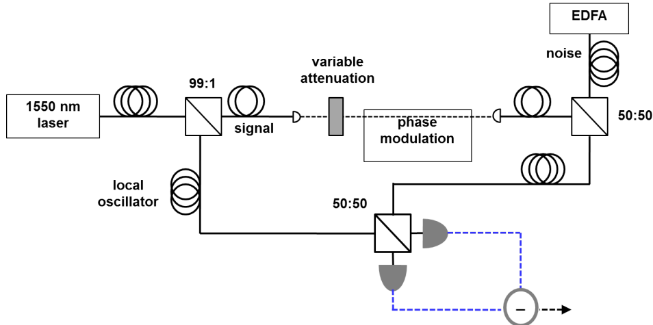
Figure 3: Schematic of classical-illumination target detection.
