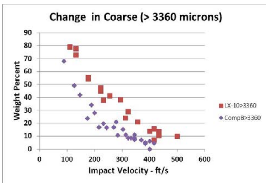
FIGURE 31. Change in Diameter Greater Than 3,360 \mu\text{m} Size Fraction.
