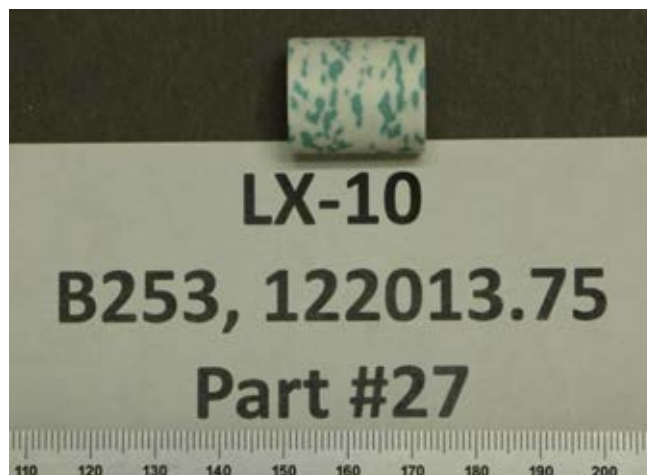
FIGURE 3. Typical Cylindrical LX-10 Friability Sample (mm Scale Divisions).
