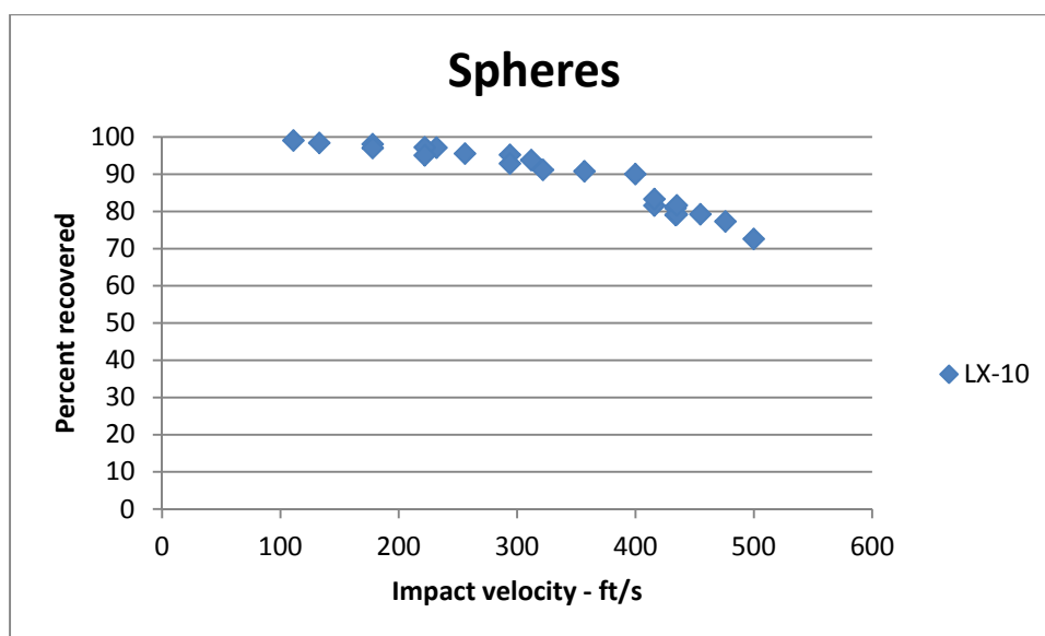
FIGURE 13. Spherical LX-10 Sample Recovered Versus Impact Velocity.
