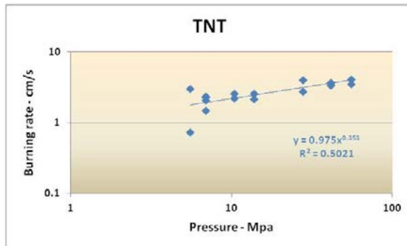
FIGURE C-28. Neat TNT Burning Rate Versus Pressure.
