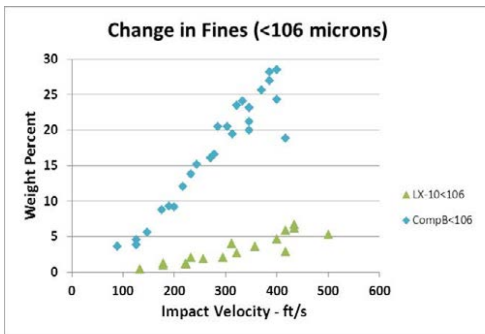
FIGURE 32. Change in Fine Particles Less Than 106 \mu\text{m} Size Fraction.
