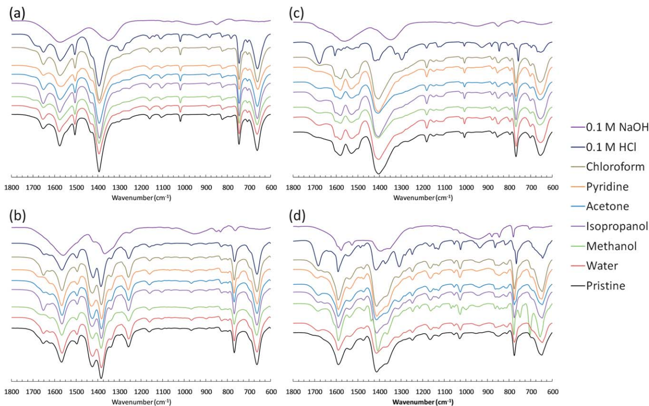
Fig. 7 ATR-FTIR spectra from 1800 to 600 \text{cm}^{-1} of (a) ZrMOF-BDC, (b) -NH 2 , (c) -BPDC, and (d) -BIPY as synthesized and after exposure to a variety of chemicals.
