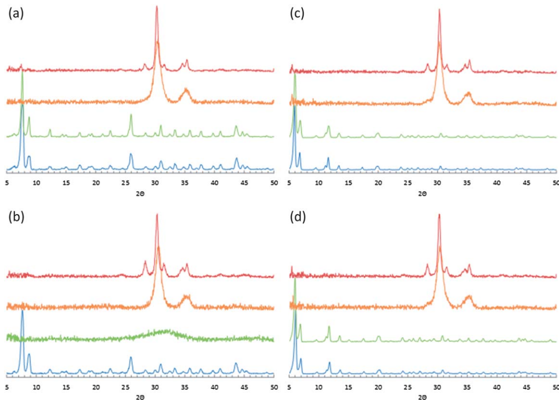
Fig. 4 PXRD spectra from 2\theta = 5 to 50^\circ of (a) ZrMOF-BDC, (b) ZrMOF-NH 2 , (c) ZrMOF-BPDC, and (d) ZrMOF-BIPY as synthesized (blue) and after heating to 350 °C (green), 550 °C (orange), and 800 °C (red) for 2 hours in air.
