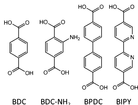
Fig. 1 ZrMOF syntheses use 1,4-benzene dicarboxylic acid, 2-aminoterephthalic acid, biphenyl-4,4'-dicarboxylic acid, and 2,2'-bipyridine-5,5'-dicarboxylic acid (left to right) as organic linkers in ZrMOF-BDC, ZrMOF- NH_2 , ZrMOF-BPDC, and ZrMOF-BIPY respectively.
