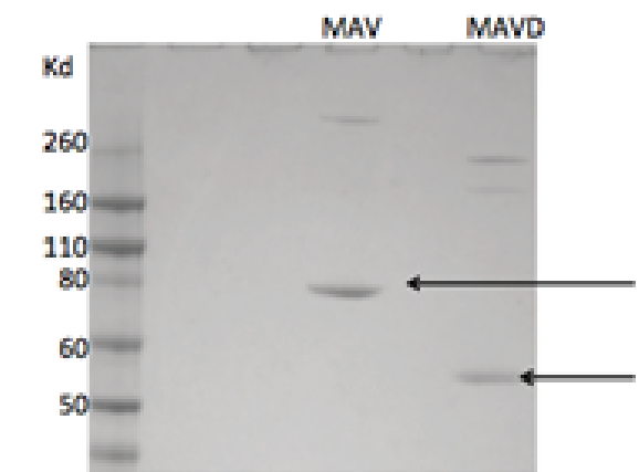
Figure 7. Molecular Weight and Purity of MAV and MAVD on Gel Electrophoresis
