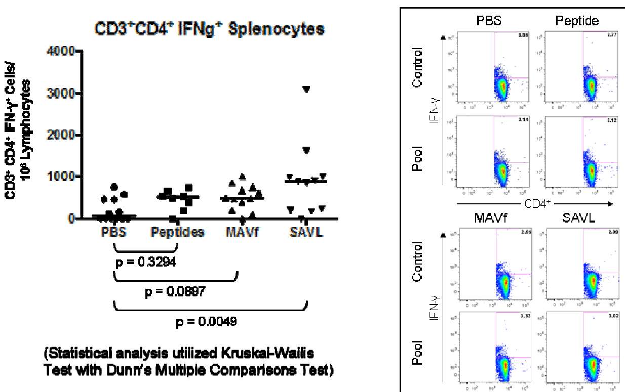
Figure 5: Lassa Vaccine Induces a Significant Increase in ^+IFN-\gamma from CD4^+ T Cells in Response to Class II Lassa Peptide Stimulation
