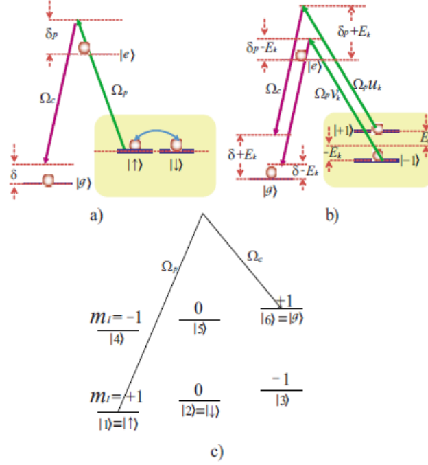
FIG. 2: (a) The bare state picture of our model. (b) The dressed state picture of our model equivalent to (a). (c) A possible realization in {}^6\text{Li} . Here the states labelled by |i\rangle ( i = 1, 2, \dots, 6 ) are the 6 ground state hyperfine states. Most experiments involving {}^6\text{Li} are performed with a magnetic field strength tuned near a Feshbach resonance at 834G. Under such a magnetic field, the magnetic quantum number for the nuclear spin m_I is, to a very good approximation, a good quantum number. The values of m_I are shown in the level diagrams. Two-photon transition can only occur between states with the same m_I . Any pair of the lower manifold ( |1\rangle , |2\rangle , and |3\rangle ) can be chosen to form the pairing states. In the example shown here, we choose |1\rangle = |\uparrow\rangle , |2\rangle = |\downarrow\rangle and |6\rangle = |g\rangle . The excited state |e\rangle (not shown) can be chosen properly as one of the electronic p state.
