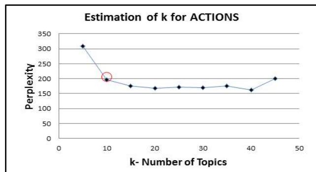
Figure 4. Number of Topics for ACTIONS, Estimated Using Perplexity Measure
