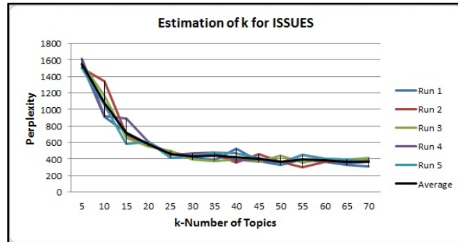
Figure 3. Number of Topics for ISSUES Estimated Using Perplexity Measure
