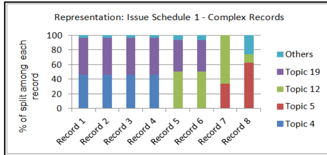
Figure 10. Complex Records, Records With Probability to Belong to Different Topics
