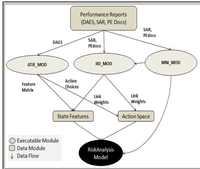
Figure 1. Decision Support Architecture for MDAP Cascading Risk Analysis Automated Text & Image Extraction Module (ATIE_MOD)
