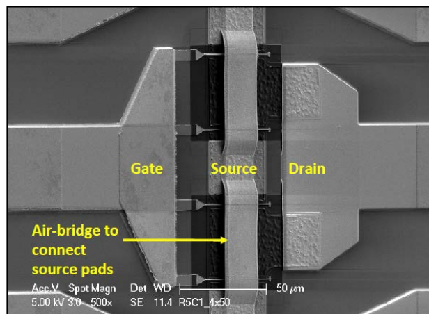
Figure 1. Scanning Electron Microscope (SEM) Image of 4 \times 50 \mu\text{m} HEMT with Four gate Fingers, Each 50\text{-}\mu\text{m} Wide
