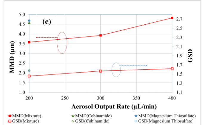
Fig. 4 Measured aerosol sizes in mass median diameter (MMD)/geometrical standard deviation (GSD) versus output rate for 100mM cobinamide solution and 1 M magnesium thiosulfate solution using the 2 MHz 4-Fourier horn ultrasonic nebulizers with (a) single-nozzle, and (b) and (c) twin-nozzle. Note that all data in (b) and (c) were obtained at a distance of 7 cm from the nozzle end face.
