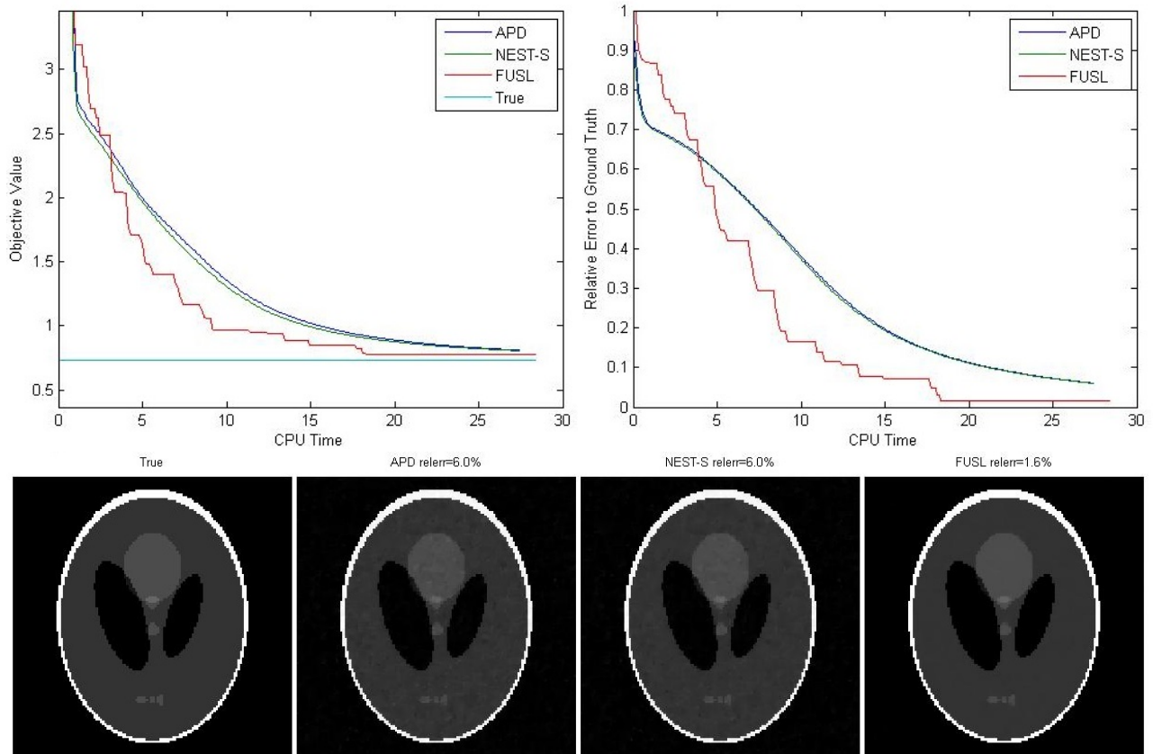
FIG. 5.1. TV-based reconstruction (Shepp-Logan phantom)
