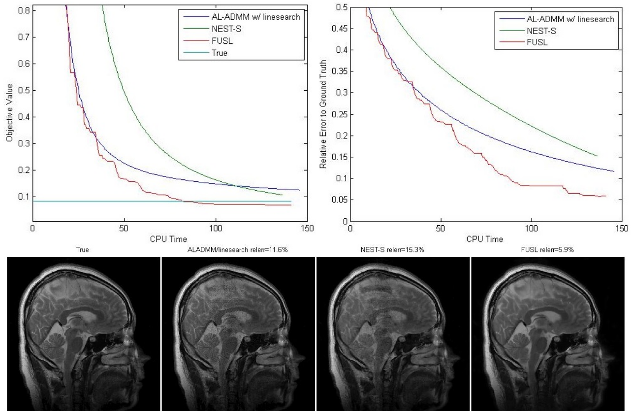
FIG. 5.4. PPI image reconstruction (acquisition rate: 14%)
