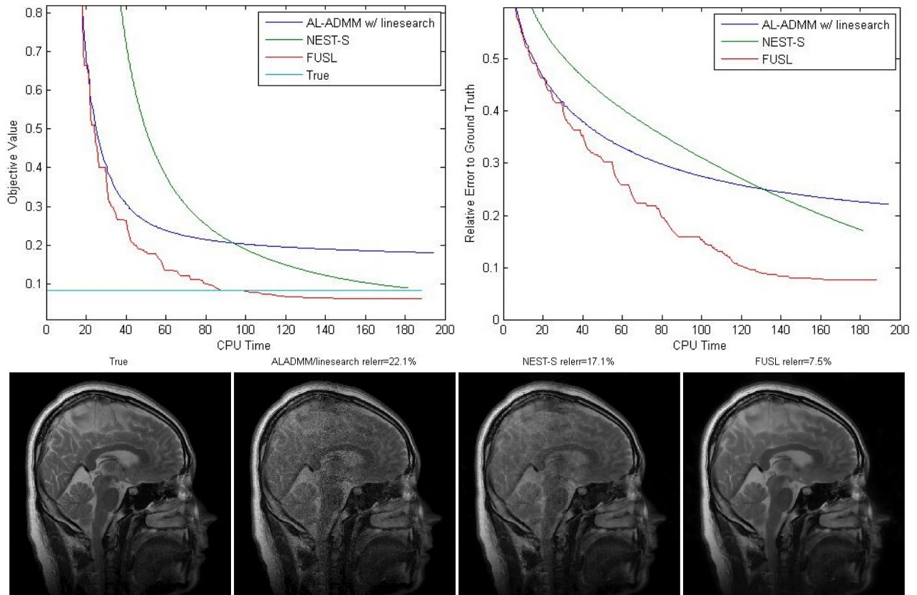
FIG. 5.5. PPI image reconstruction (acquisition rate: 10%)
