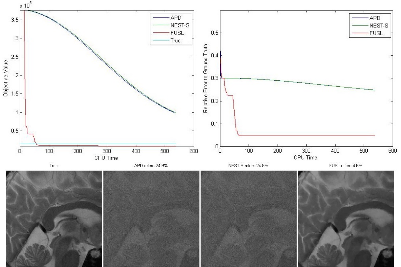
FIG. 5.2. TV-based reconstruction (brain image)
