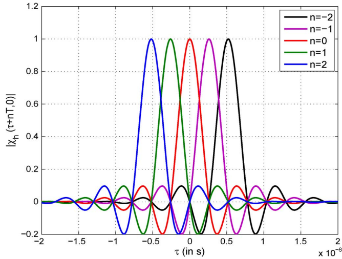
Fig. 2. |\chi_h(nT + \tau, 0)| for different n as a function of \tau .
