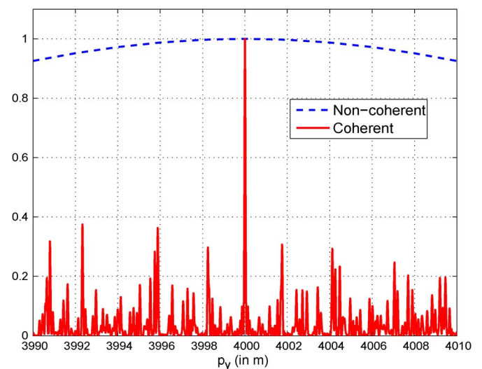
Fig. 11. Coherent and non-coherent ambiguity functions in the y-position dimension.
