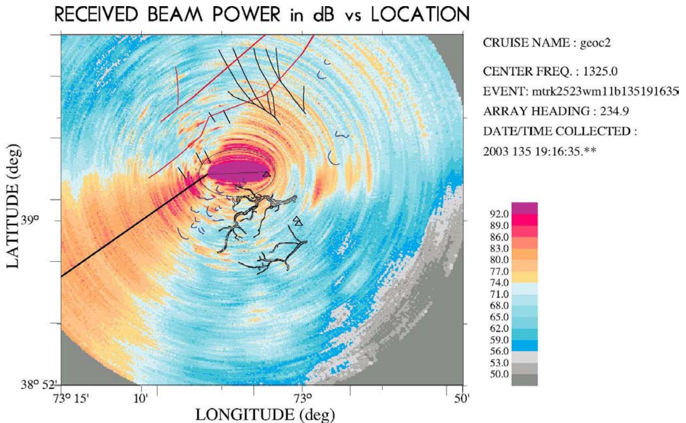
Fig. 1. Polar plot of the bistatic reverberation on the FORA cardioid array from a 1s LFM pulse near STRATAFORM, Site S2 in the 1250--1400 Hz band. The black line to the southwest indicates the array heading. The array is at the start of that line. The source is located at the right end of the horizontal line from the receiver (at the triangle). Levels indicated by color scale are in dB//1uPa 2 /Hz. Left-right ambiguity is broken by the cardioid beamformer and shows excellent left-right rejection on various clutter features (most likely fish schools [11]).
