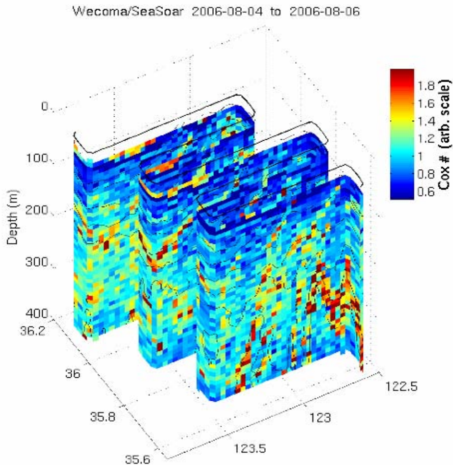
Figure 5. The Cox number approximation is plotted on a log scale and contours are salinity at 0.1 psu intervals. Mixing appears to be higher in shear zones between different water masses on the east side of the front and along a subducting, tilted isopycnal where current shear is high. Data are over a smaller lateral extent and a larger vertical extent than Figures 3-4.
