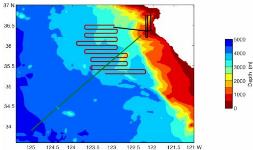
Figure 1. The cruise consisted of 3 segments near Monterey Bay: a front survey (red), an offshore line (green), and an internal tide survey (black). R/P FLIP was moored between our east and central internal tide lines. The front was located ~100 km offshore and the survey had thirteen cross-front legs, which are ~70 km long and separated by 11 km. The offshore line extended ~400 km offshore from Point Sur and was perpendicular to the coast. The internal tide survey repeated three lines near Sur Platform about twenty times and an offshore line four times.
