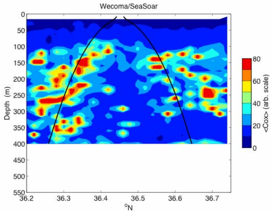
Figure 7. Mean Cox number in a meridional depth section is calculated from \sim 20 repeat lines, which are obtained by combining about six repeats of the three north-south lines across Monterey Canyon. Higher mean values appear to be found along M2 characteristics (black lines). □
